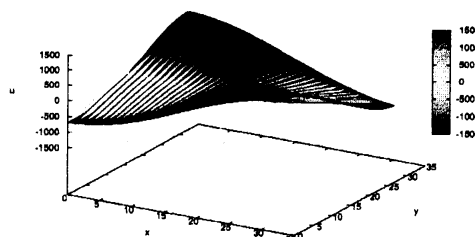
FIGURE 3. \mu = 100.0, t = 3200
