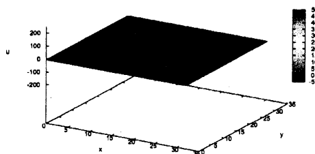
FIGURE 1. t = 0
