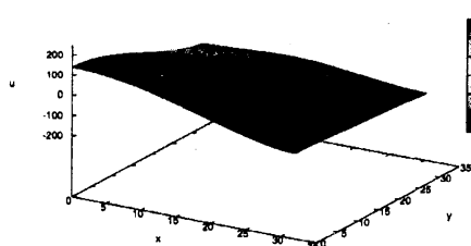
FIGURE 2. \mu = 1.0, t = 6000
