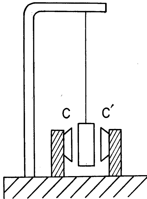
Fig. 1 Variable capacitance-transducer (schematic).
