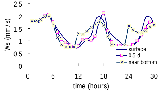
Fig. 9 Computed variations in settling velocity.
