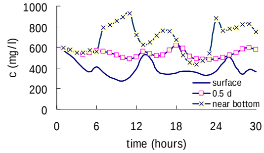
Fig. 8 Computed variations in concentration.
