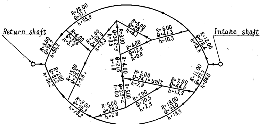
Fig. 3. Examples of Ventilation Networks Solved with Two Unknowns.
