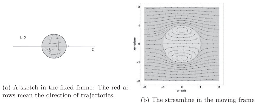
Figure 1: An illustration of Hill's vortex
