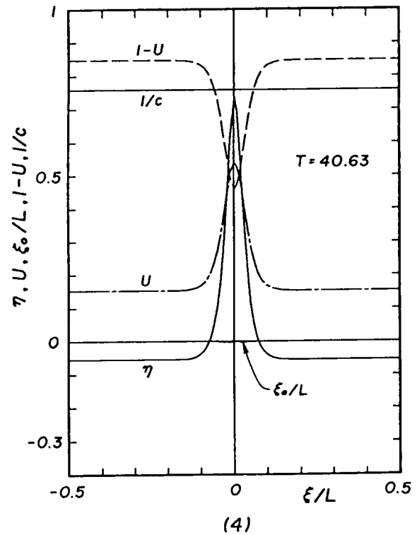
Fig. 4.30 Wave profiles and distributions of average velocity with respect to the phase of waves ( Q = 0.8 , R = 10^8 , s = 0.00182 ).
