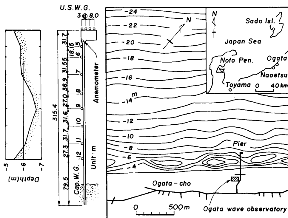
Fig. 4.48 Environments of a observational pier and linear wave-probe array.
