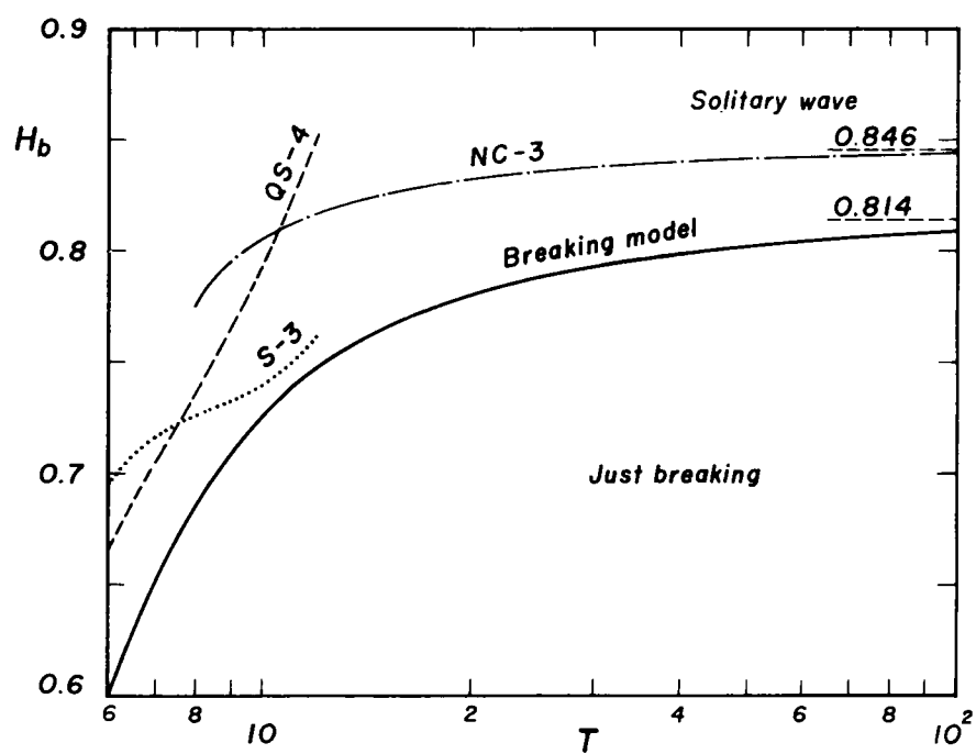
Fig. 2.12 Changes in wave height at just breaking.
