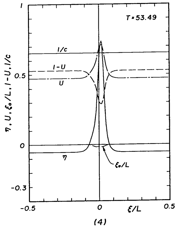
Fig. 4.26 Wave profiles and distributions of average velocity with respect to the phase of waves ( \bar{Q} = 0.5 , R = 10^7 , s = 0.00303 ).
