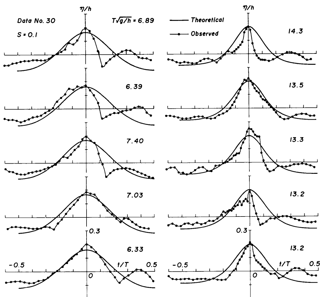
Fig. 4.62 Comparison of wave profiles of the wind-forced waves with theoretical ones (Data No. 30).
