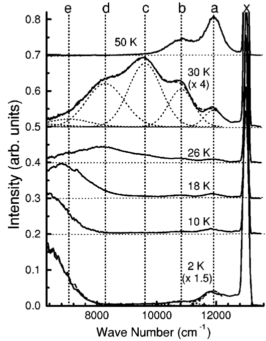
FIG. 1. Emission spectra of \text{K}^*\text{He}_n in the case of D_2 excitation at various temperatures in gaseous He (solid lines). They are normalized by the total intensity integrated over \nu > 6300 \text{ cm}^{-1} . The superposition curves (dashed lines) of five Gaussian curves and the emission spectrum of \text{K}^*\text{He}_{n_{\text{max}}} in liquid He (dotted lines) are fitted to the spectra observed at 2 K and 30 K. Vertical dotted lines labeled as a-e indicate the peak positions of the five Gaussian curves for n=1-5 , respectively. Sharp emission line labeled as x is the D emission line of atomic K.
