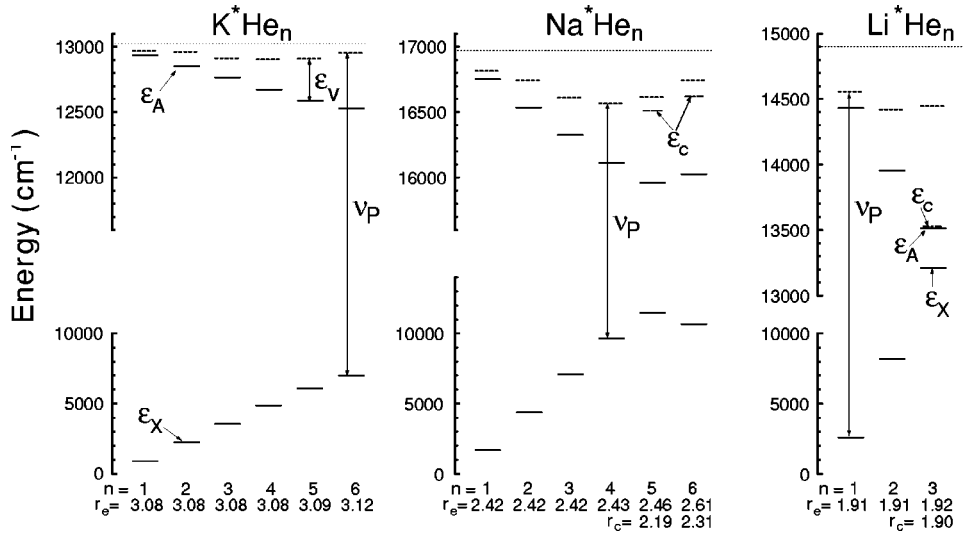
FIG. 7. Theoretical values of \epsilon_A (solid lines), \epsilon_X (solid lines), and \epsilon_A + \epsilon_v (dashed lines) of each exciplex M^*\text{He}_n . The equilibrium radius r_e (in Å) is also shown. The dotted lines indicate the spin-orbit-averaged energy levels of the first excited P state of alkali-metal atoms relative to the level of the ground S state. The energy \epsilon_c (dash-dotted lines) and the radius r_c (in Å) at the level crossing point are shown for \text{Na}^*\text{He}_n ( n=5,6 ) and \text{Li}^*\text{He}_3 . The energy differences labeled as \nu_P indicate approximate values of peak positions of emission spectra of the exciplexes.
