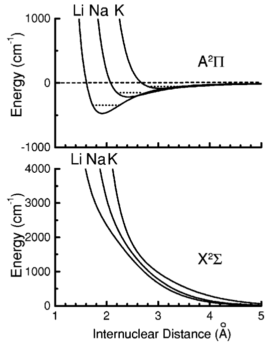
FIG. 6. Theoretical adiabatic potential curves for the A^2\Pi and X^2\Sigma states of K-He, Na-He, and Li-He obtained with the RHF calculation. The dotted lines show the energies of the rovibrational ground states. The spin-orbit coupling is not included. The zero energy corresponds to the energy at the dissociation limit.
