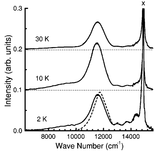
FIG. 5. Emission spectra of \text{Li}^*\text{He}_n at various temperatures in gaseous He (solid lines). The dashed line is the best-fitted superposition of theoretical emission spectra from different vibrational states of \text{Li}^*\text{He} . Sharp emission line labeled as x is the D emission line of atomic Li.
