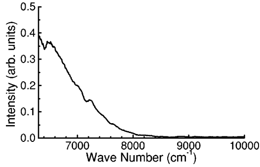
FIG. 2. Emission spectrum of K^*He_{n_{\max}} in liquid He.
