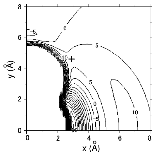
FIG. 8. Potential-energy surface calculated for the system of \text{K}^*\text{He}_2\text{-He} including the spin-orbit coupling. The K atom is fixed at (x,y)=(0,0) and the two He atoms of \text{K}^*\text{He}_2 are fixed at (0, \pm 3.08) in unit of Å. The energy in unit of \text{cm}^{-1} is measured from the dissociation limit \text{K}^*\text{He}_2(\tilde{A}^2\Pi_{1/2})+\text{He} . The contour interval is 5\text{ cm}^{-1} . The marks “+” and “x” indicate the positions of the saddle point and the potential minimum, respectively.
