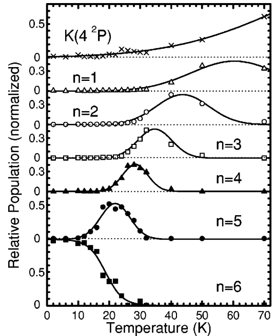
FIG. 3. Temperature dependence of the relative populations for K^*He_n ( n=1-6 ) and K(4^2P) . Solid lines are guides for the eye.
