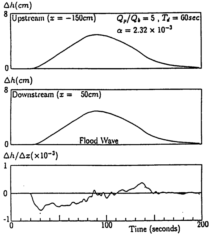
Fig. 3 Profiles of flood surface wave measured simultaneously at two points ( \Delta x = 200\text{ cm} ).
