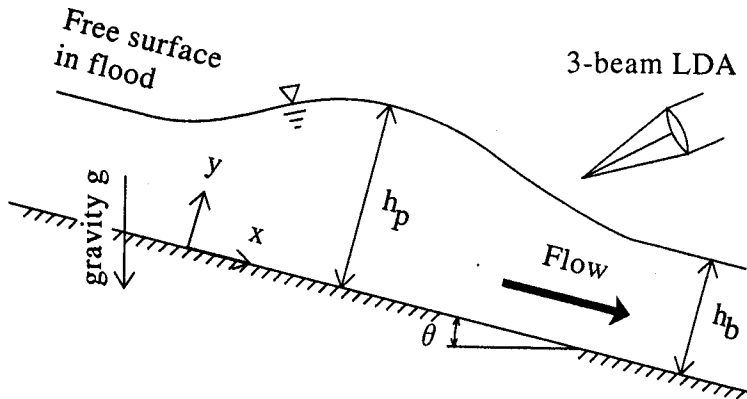
Fig. 1 Schematic description of unsteady free-surface flow. Even the depth-varying zone h_b < y < h_p can be measured accurately with LDA.
