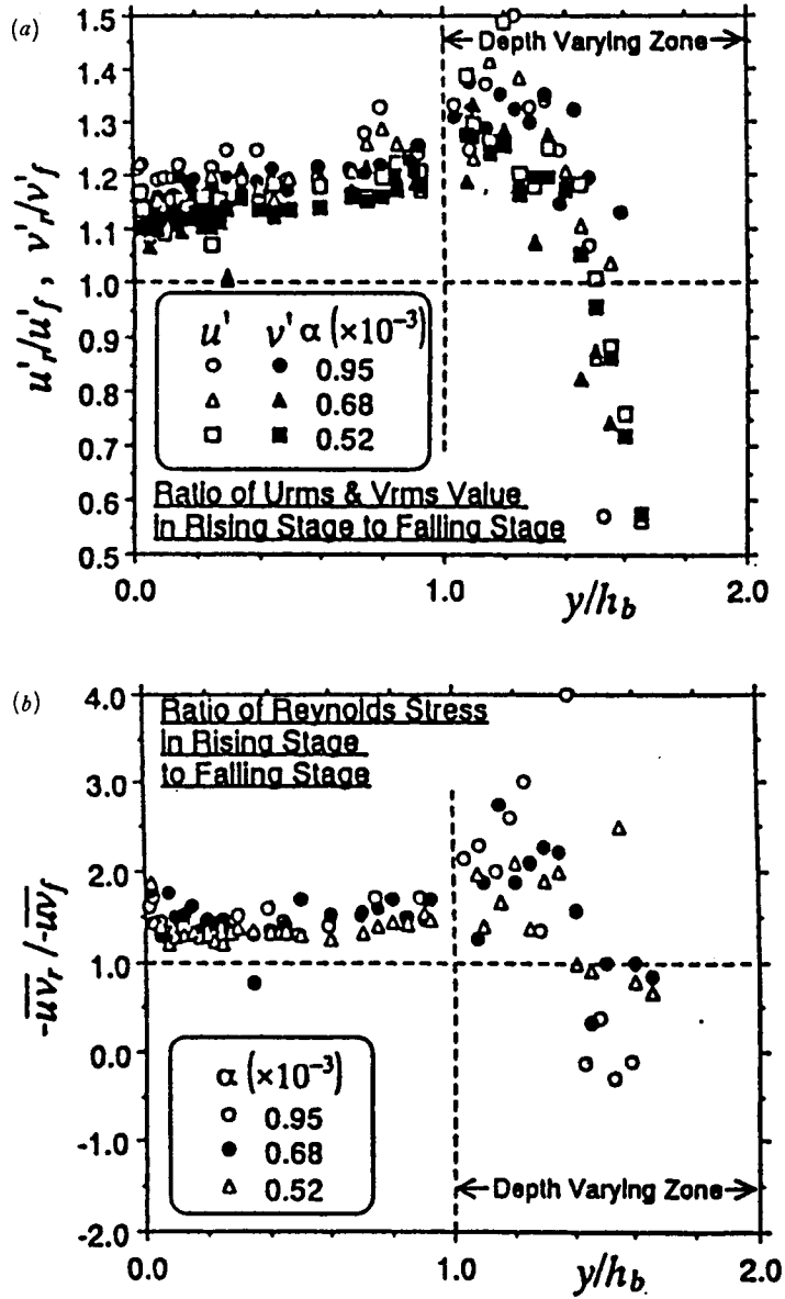
Fig. 16 The ratio turbulence of the rising flood stage to that of the falling one. (a) turbulence intensities u'/u_f and v'/v_f , and (b) Reynolds stress -\overline{u'v_r}/-\overline{u'v_f} .
