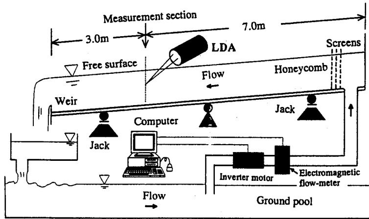
Fig. 2 Schematic description of experimental flume and water circulation system.
