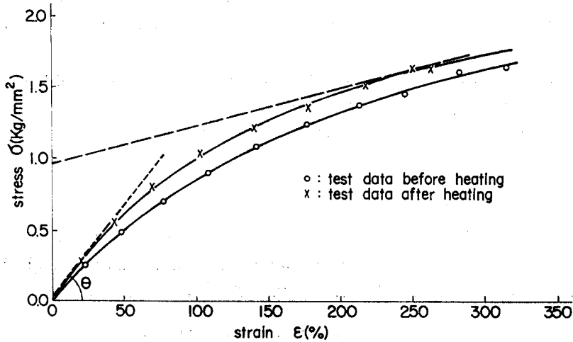
Fig. 3 Stress-strain relation
