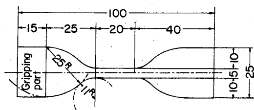
Fig. 1 Specimen of dumb-bell shape No. 3 Unit : mm
