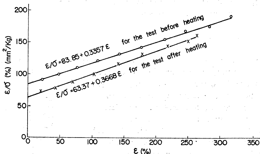
Fig. 5 Relation between strain/stress and strain
