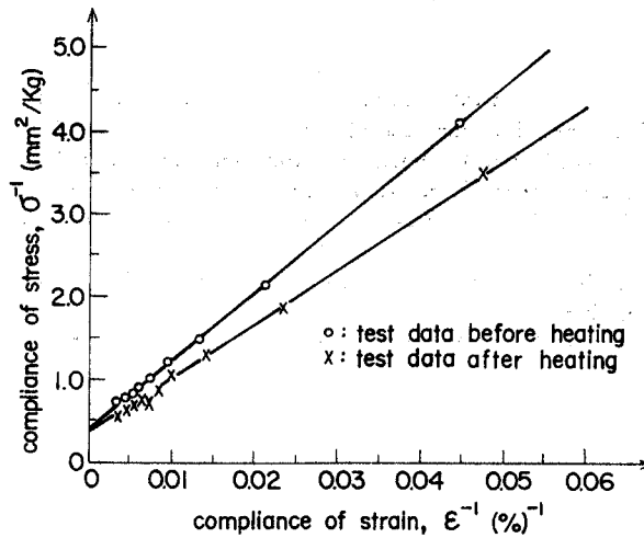
Fig. 6 Relation between compliance of stress ( \sigma^{-1} ) and compliance of strain ( \epsilon^{-1} )
