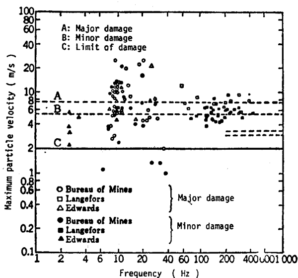
Fig. 13. Relation between Particle Velocity and Damage Observed by U.S. Bureau of Mines.
