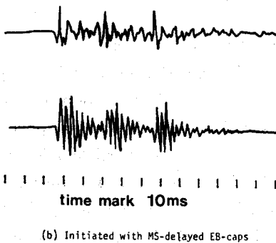
Fig. 17. Oscillogram of Blasting Vibration
