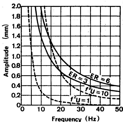
Fig. 14. Allowable Limit Specified by Energy Ratio
