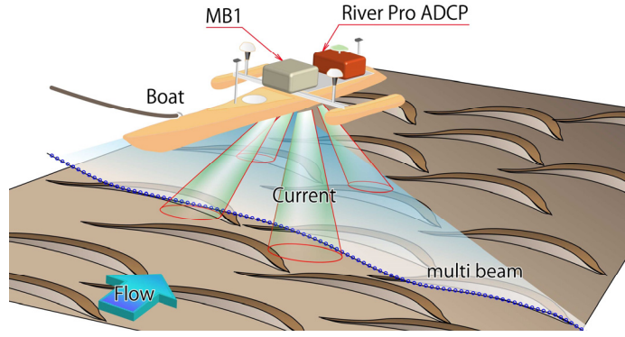
Figure 2: Sketch of measurement system
