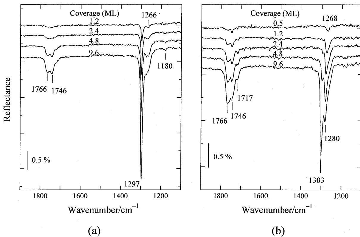
Figure 6.5 IRA spectra of \text{N}_2\text{O}_4 adsorbed at 91 K as a function of \text{N}_2\text{O}_4 coverage on (a) 8-ML crystalline ice and (b) 5-ML semicrystalline ice.
