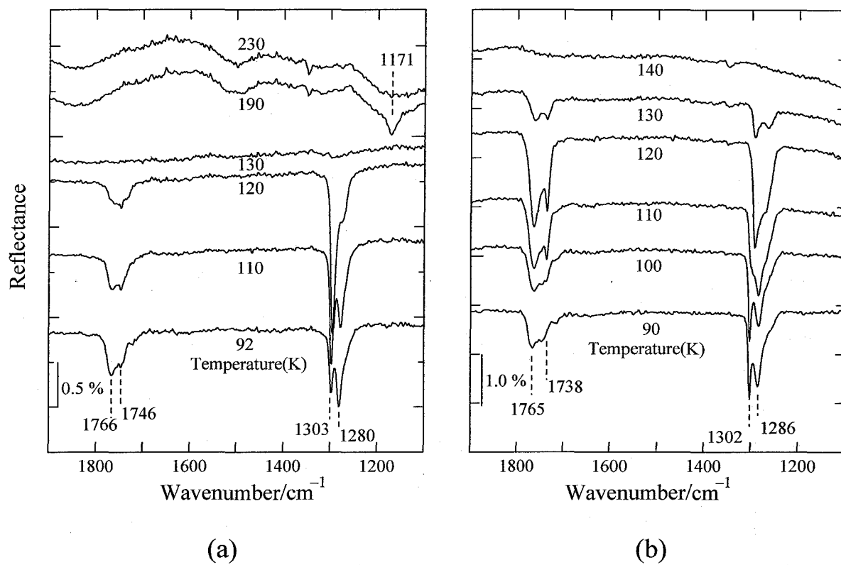
Figure 6.7 Temperature dependence of the IRA spectrum of \text{N}_2\text{O}_4 adsorbed on (a) 5 ML semicrystalline ice and (b) 3 ML amorphous ice. The substrate temperature was elevated stepwisely to the indicated temperatures.
