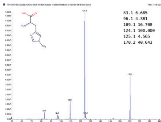
Fig. 1. Example MS spectrum from Human Metabolome Database (Wishart et al., 2012) for 1-Methylhistidine (HMBD00001), with its corresponding chemical structure (top-left) and peak list (top-right)
