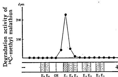
Fig. 1. Degradation of ^{14}\text{C} -methyl malathion by the smaller brown planthopper enzymes of LE strain separated by agar-gel electrophoresis. The agar plate was sliced into 5 \times 50 mm pieces and each agar piece was incubated at 37^\circ\text{C} for 2 hr with 10^{-8}\text{M} of ^{14}\text{C} -methyl malathion to assess its degradation activity. The corresponding zymogram for \beta -naphthyl acetate indicates the relative positions of esterase bands against malathion degrading enzyme.
