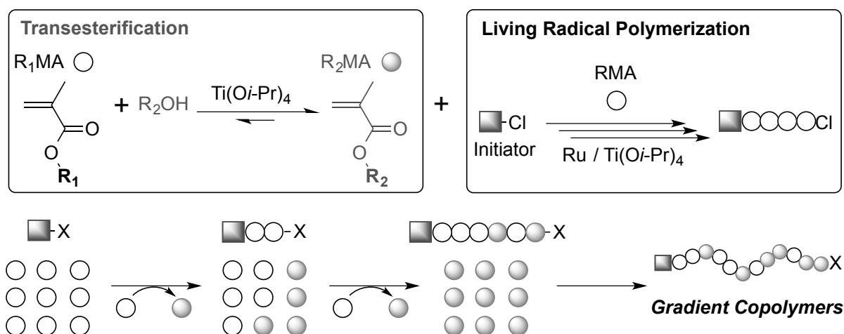
Figure 7. Concurrent tandem catalysis of transesterification and living radical polymerization.
