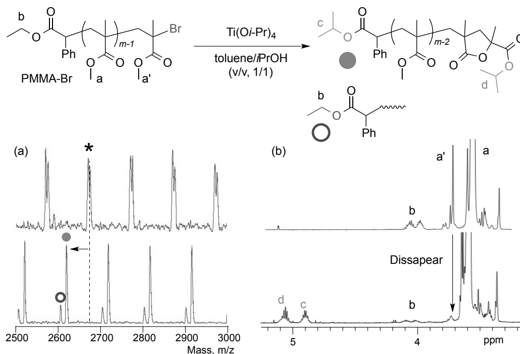
Figure 3. Concurrent cyclization and transesterification of Et-PMMA-Br: [\text{Et-PMMA-Br}]/[\text{Ti}(\text{Oi-Pr})_4] = 20/40 mM in toluene/ i\text{PrOH} (1/1, v/v) at 80^\circ\text{C} for 48h: (a) MALDI-TOF-MS and (b) ^1\text{H} NMR ( [\text{Polymer}] = 10 mg in \text{CD}_2\text{Cl}_2 at 25^\circ\text{C} ) spectra of PMMA-Br (upper) and the product (lower).
