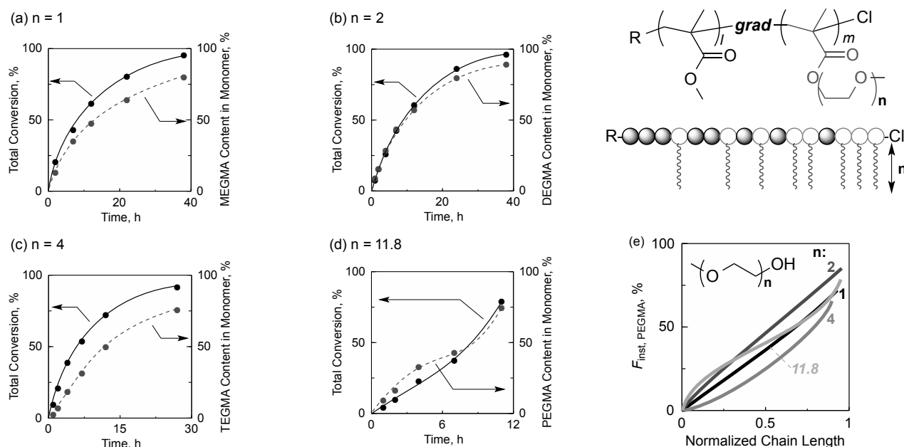
Figure 4. Synthesis of MMA/PEGMA gradient copolymers via concurrent tandem catalysis with various PEG-OH [ \text{CH}_3(\text{OCH}_2\text{CH}_2)_n\text{OH} : n = 1, 2, 4, 11.8 ( M_n = 550 )] : [\text{MMA}]/[\text{ECPA}]/[\text{Ru}(\text{Ind})\text{Cl}(\text{PPh}_3)_2]/[\text{Ti}(\text{Oi-Pr})_4] = 1000/5/1/20 ( n = 1, 2, 4 ) or 40 ( n = 11.8 ) mM in toluene/PEG-OH (1/1, v/v) with MS 4A (0.33 g/mL) at 80^\circ\text{C} . (a)-(d) total monomer conversion and PEGMA content in monomer as a function of time: (a) n = 1 (b) 2 (c) 4 (d) 11.8 . (e) Instantaneous PEGMA composition in copolymers obtained with each alcohol.
