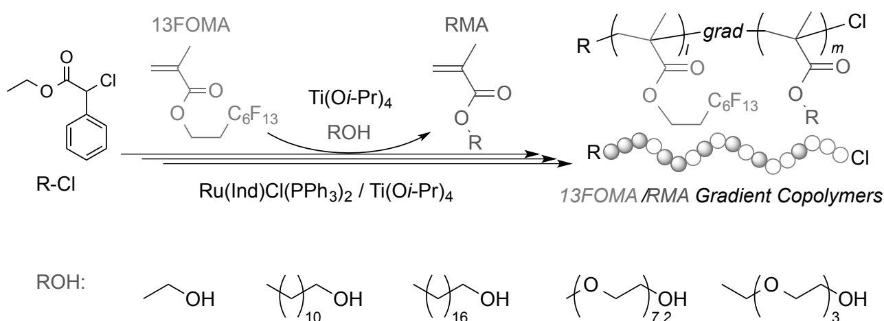
Scheme 1. Synthesis of Fluorous, Perfluorinated Gradient Copolymers via Tandem Catalysis of Living Radical Polymerization and Transesterification of 13FOMA with Various Alcohols
