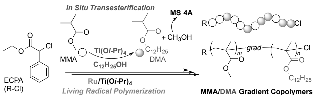
Scheme 3. MMA/DMA Gradient Copolymers via Concurrent Tandem Catalysis of LRP and In-Situ Transesterification of MMA with 1-Dodecanol
