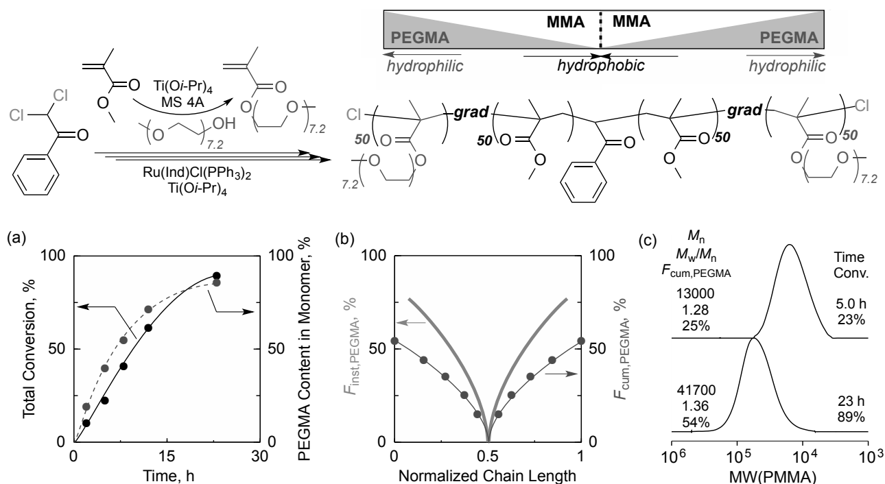
Figure 5. Synthesis of a MMA/PEGMA bidirectional gradient copolymer via concurrent tandem catalysis with 2,2-dichloroacetophenone (DCAP): [\text{MMA}]/[\text{DCAP}]/[\text{Ru}(\text{Ind})\text{Cl}(\text{PPh}_3)_2]/[\text{Ti}(\text{Oi-Pr})_4] = 1000/5/1/20 mM in toluene/PEG-OH ( M_n = 350 ) (1/1, v/v) with MS 4A (0.33 g/mL) at 80 °C.
