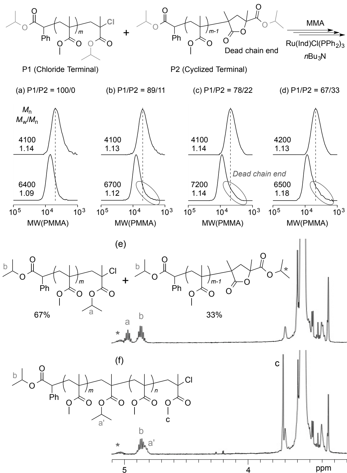
Figure 4. Chain extension from P1/P2 mixture via LRP of MMA: [\text{MMA}]/[\text{P1+P2}]/[\text{Ru(Ind)Cl(PPh}_3)_2]/[n\text{-Bu}_3\text{N}] = 500/10/1/10 mM in toluene at 80 °C. SEC curves of products obtained from (a) P1/P2 =100/0 (b) 89/11 (c) 78/22 (d) 67/33. 1 H NMR spectra of (e) P1/P2 mixture and (f) the product: [polymer] = 10 mg/mL in CD 2 Cl 2 at 25 °C.
