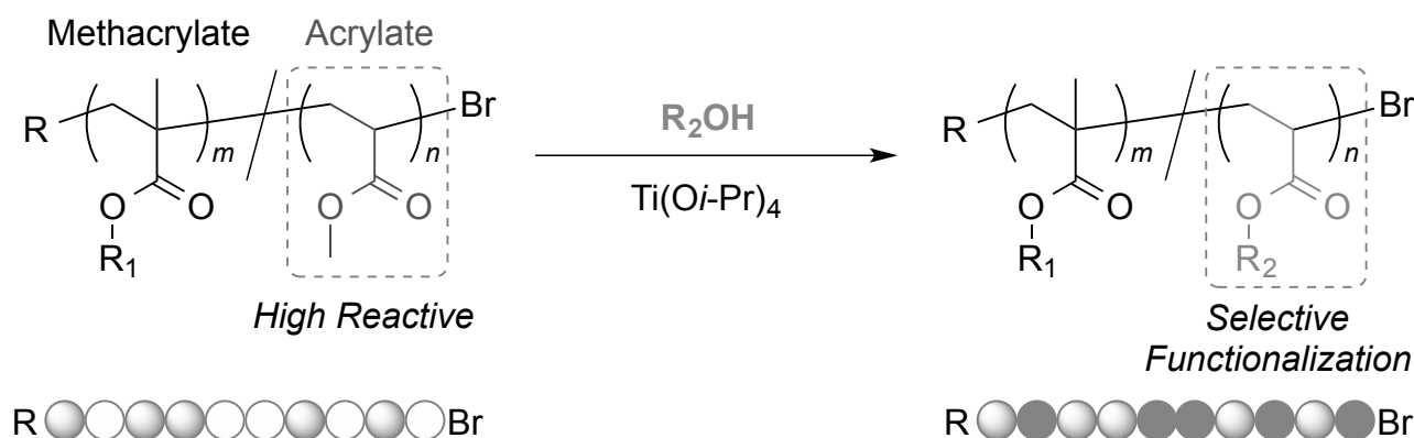
Scheme 1. Acrylate-Selective Transesterification of Methacrylate/Methyl Acrylate ( \text{R}_1\text{MA/MA} ) Random Copolymers with Alcohols ( \text{R}_2\text{OH} ) into \text{R}_1\text{MA/R}_2\text{A} Random Copolymers
