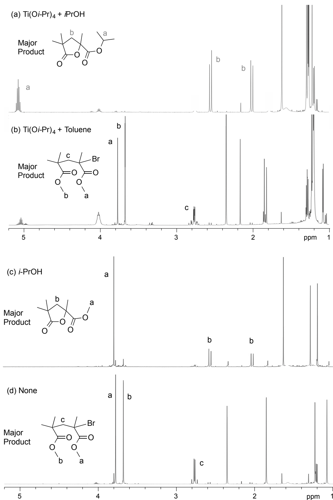
Figure 2. Effects of Ti catalyst and i\text{PrOH} on cyclization of \text{H}(\text{MMA})_2\text{-Br} : [\text{H}(\text{MMA})_2\text{-Br}]/[\text{Ti}(\text{O}i\text{-Pr})_4] = 20/0 (c,d) or 40 (a,b) mM in toluene/ i\text{PrOH} (1/1, v/v) (a,c) or toluene (b,d) at 80 °C for 46h. ^1\text{H} NMR spectra of their products in \text{CDCl}_3 at 25 °C.
