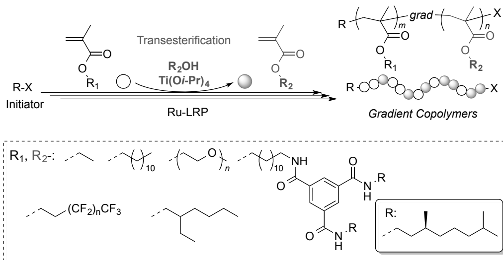
Scheme 1. Concurrent Tandem Catalysis of LRP and Monomer-Selective Transesterification for Functional Gradient Copolymers
