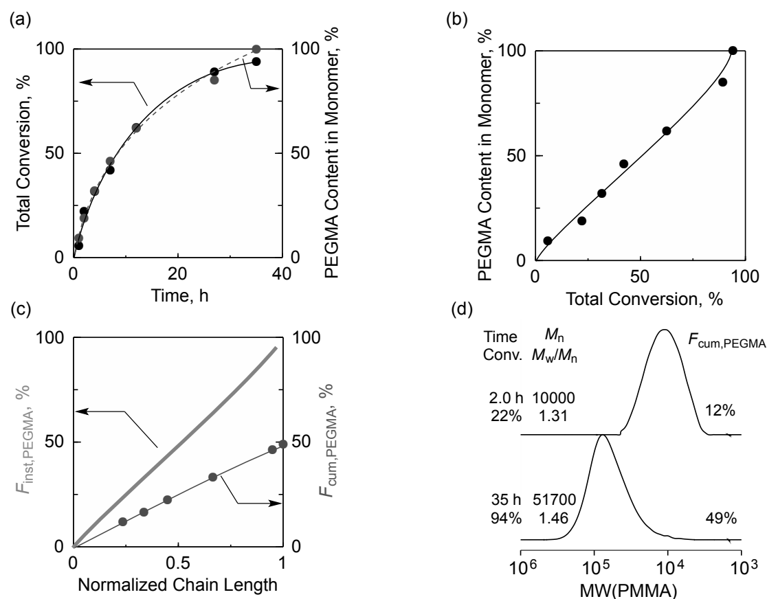
Figure 1. Synthesis of MMA/PEGMA gradient copolymers via concurrent tandem catalysis: [\text{MMA}]/[\text{ECPA}]/[\text{Ru}(\text{Ind})\text{Cl}(\text{PPh}_3)_2]/[\text{Ti}(\text{Oi-Pr})_4] = 1000/5/1/20 mM in toluene/PEG-OH ( M_n = 350 ) (1/1, v/v) with MS 4A (0.33 g/mL) at 80 °C. (a) total monomer conversion and PEGMA content in monomer. (b) PEGMA content in monomer as a function of total conversion. (c) cumulative ( F_{\text{cum,PEGMA}} ) and instantaneous ( F_{\text{inst,PEGMA}} ) PEGMA content in products. (d) SEC curves of products.
