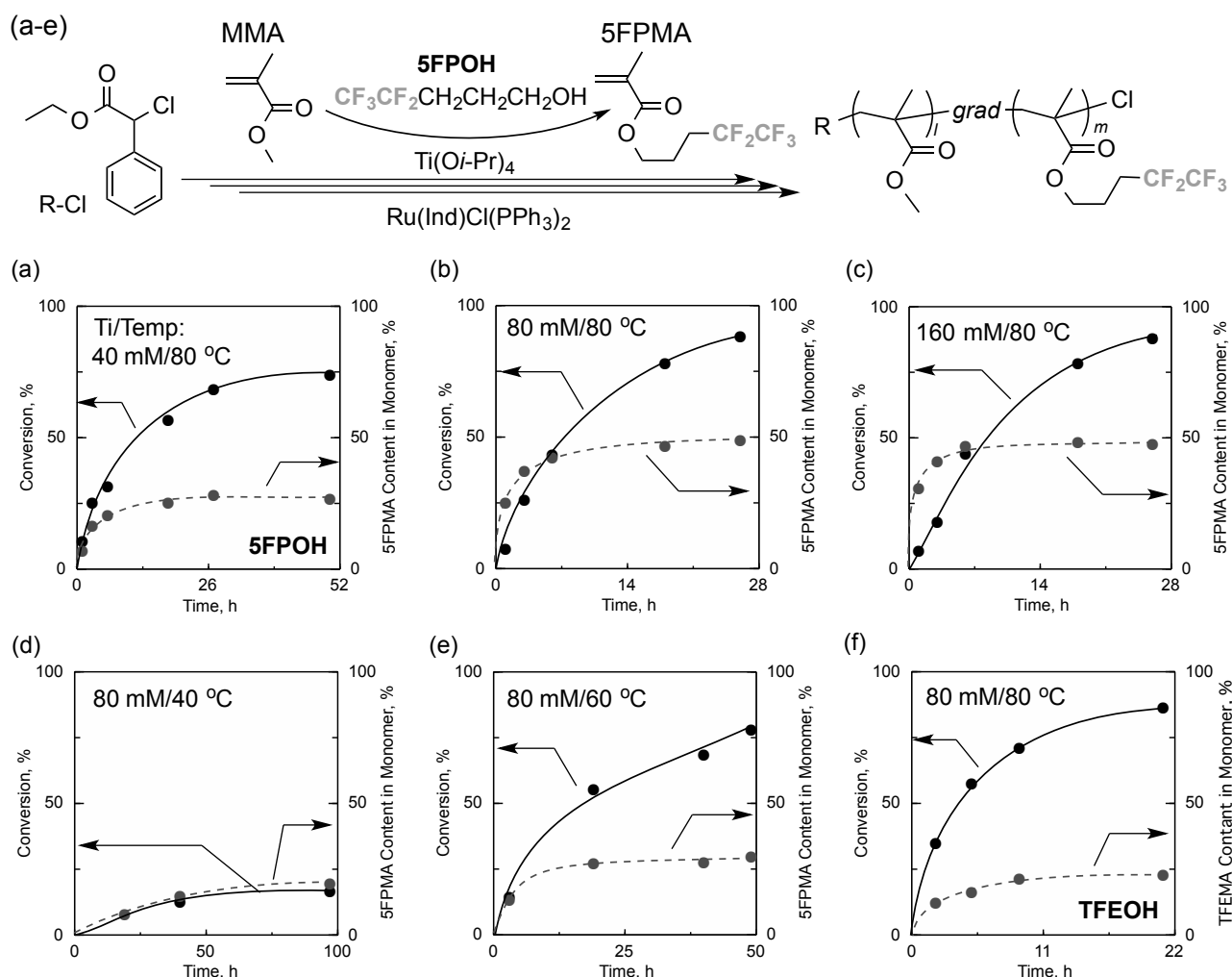
Figure 1. Tandem polymerization of MMA with 5FPOH (a-e) or TFEOH (f) by varying \text{Ti}(\text{O}i\text{-Pr})_4 concentration and temperature: [\text{MMA}]/[\text{ECPA}]/[\text{Ru}(\text{Ind})\text{Cl}(\text{PPh}_3)_2]/[\text{Ti}(\text{O}i\text{-Pr})_4] = 2000/20/2/40\text{--}160 mM in toluene/5FPOH or TFE (1/1, v/v) at 40–80 °C ( [\text{5FPOH}] = 2.9 M, [\text{TFEOH}] = 5.3 M) (a-e) Total conversion and 5FPMA content in monomer: [\text{Ti}(\text{O}i\text{-Pr})_4]/\text{temperature} = (a) 40 mM/80 °C, (b) 80 mM/80 °C, (c) 160 mM/80 °C, (d) 80 mM/40 °C, and (e) 80 mM/60 °C. (f) Total conversion and TFEMA content in monomer: [\text{Ti}(\text{O}i\text{-Pr})_4]/\text{temperature} = 80 mM/80 °C.
