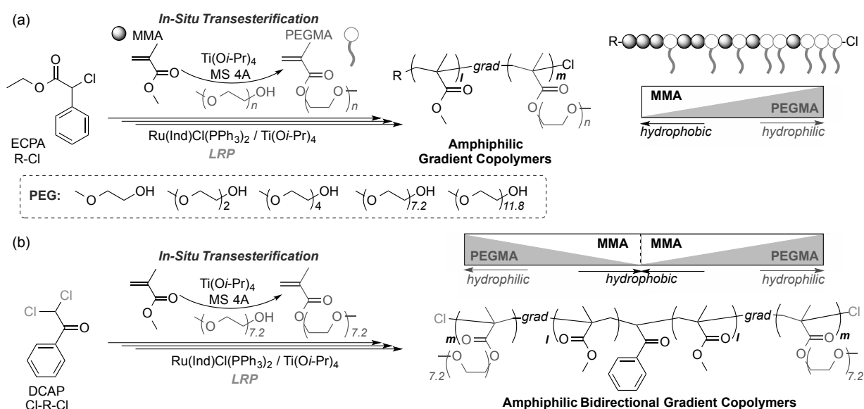
Scheme 4. Synthesis of Amphiphilic Gradient Copolymers via Concurrent Tandem Catalysis of LRP and Transesterification with MMA and Hydrophilic PEGs
