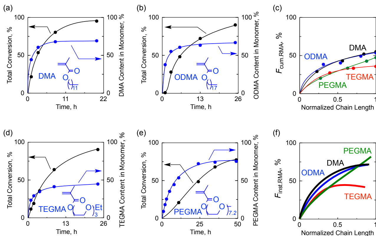
Figure 3. Synthesis of 13FOMA/RMA [RMA: DMA, ODMA, TEGMA, and PEGMA ( M_n = 350 )] gradient copolymers via concurrent tandem catalysis with 13FOMA and various alcohols: [\text{MMA}]/[\text{ECPA}]/[\text{Ru}(\text{Ind})\text{Cl}(\text{PPh}_3)_2]/[\text{Ti}(\text{O}i\text{-Pr})_4] = 1000 (PEGOH) or 2000/10 (PEGOH) or 20/2/20 mM in toluene/ROH (ROH: DOH, ODOH, TEGOH, PEGOH) (1/1, v/v) at 80 °C. (a)(b)(d)(e) total monomer conversion and RMA content in monomer. (c) F_{\text{cum,RMA}} of products as a function of normalized chain length. (f) F_{\text{inst,RMA}} of products as a function of normalized chain length.
