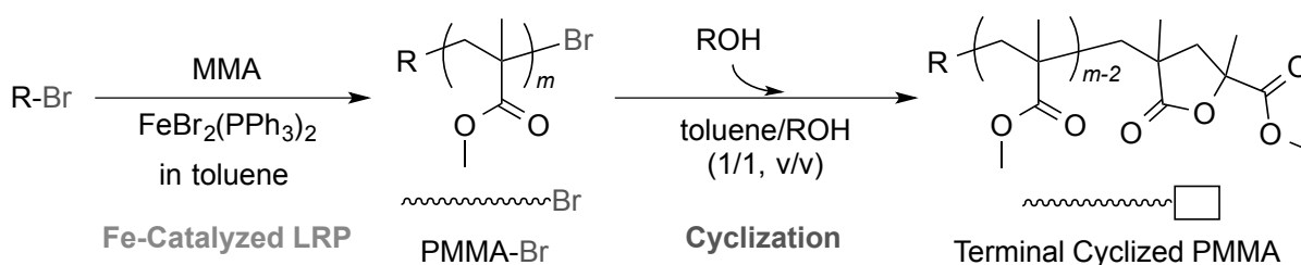
Scheme 1. (a) Concurrent and terminal-selective transesterification and intramolecular cyclization of Et-PMMA-Br with alcohols and a Ti catalyst. (b) Sequential tandem catalysis of Fe-catalyzed LRP of MMA and terminal-selective cyclization for end-cyclized PMMAs.
