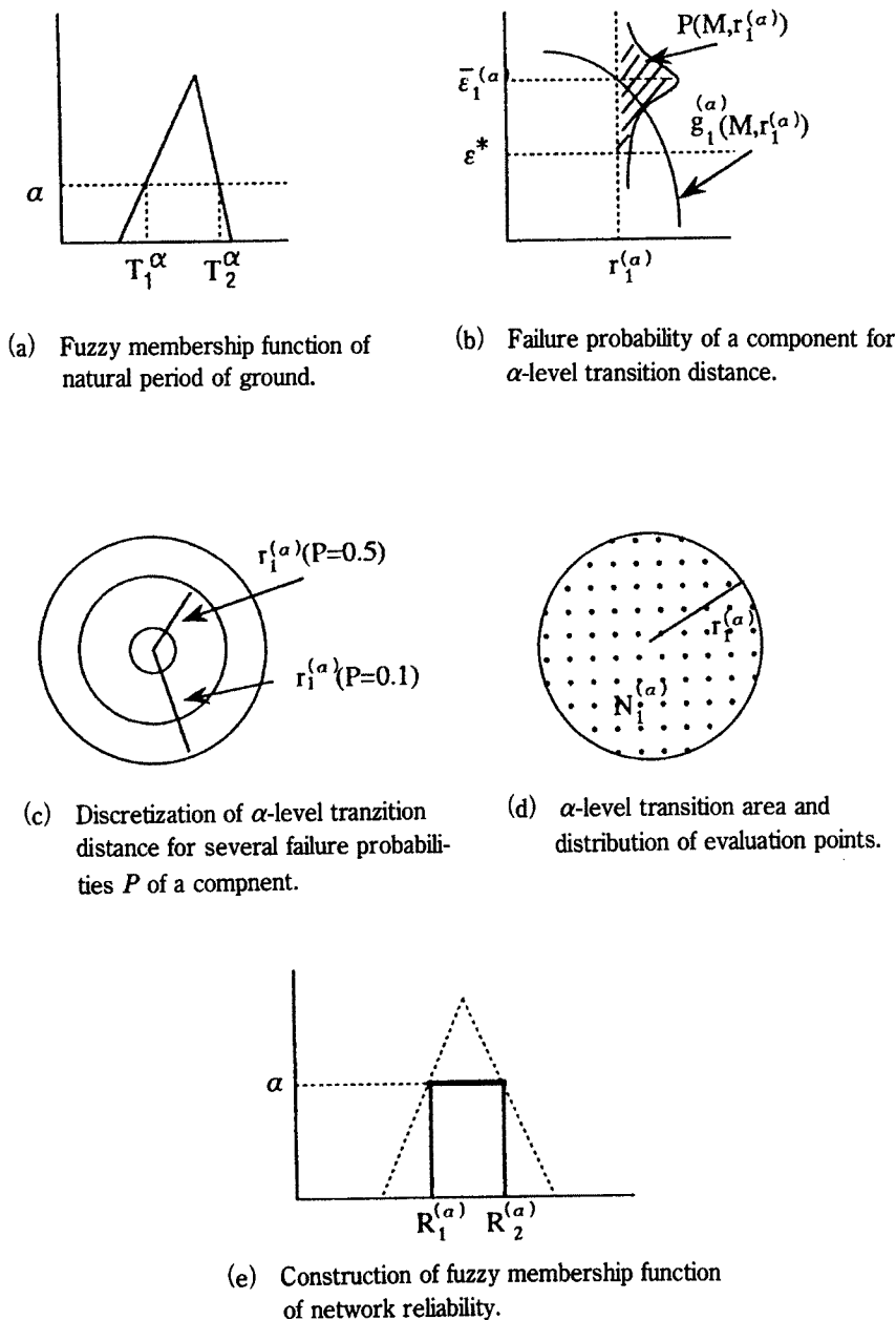
Fig. 16. Determination of fuzzy membership function of network reliability when taking into account both of the fuzzy uncertainty of natural period and probabilistic uncertainty of attenuation law of acceleration.
