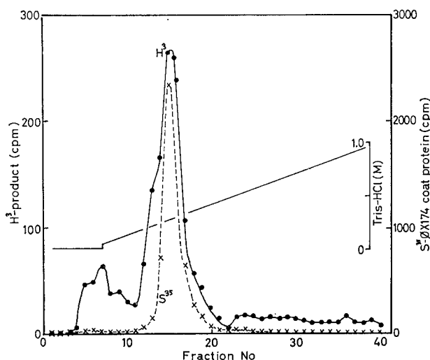
Fig. 6. DEAE-cellulose column chromatography of proteins synthesized in the "coupled system". ^3\text{H} -labelled product was chromatographed with ^{35}\text{S} -labelled authentic coat protein 31) .
