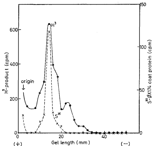
Fig. 7. Acrylamide gel electrophoresis of the proteins synthesized in the "coupled system". H^3 -labelled product was chromatographed with S^{35} -labelled authentic coat protein (28) .
