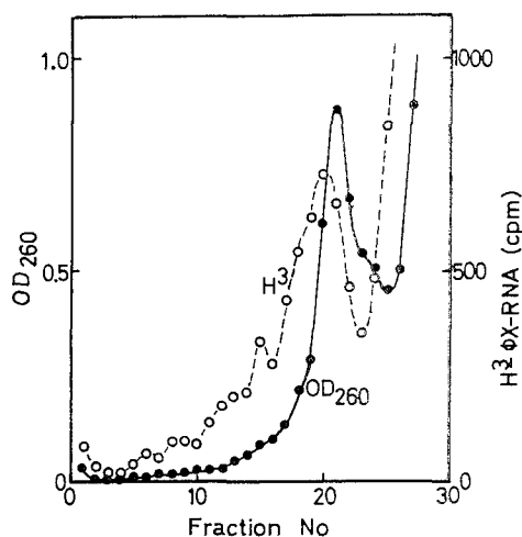
Fig. 3. Sedimentation analysis of the cell-free protein synthesizing system containing H^3 -labelled \phi X-RNA 26) .
