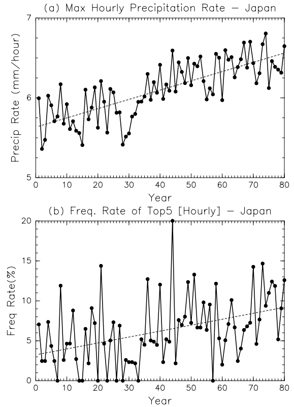
Fig. 4 The same as in Fig. 3 , except for maximum hourly precipitation rates (mm/hour).
