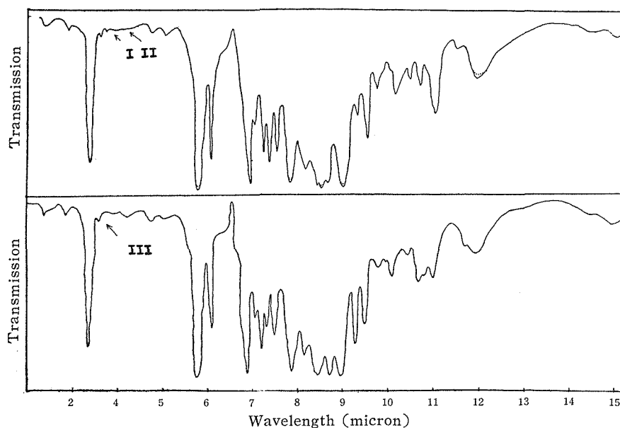
Fig. 7. Dimethylesters of naturally derived (I) and ( \pm )- trans-trans -(superimposed II) and ( \pm )- cis-trans -chrysanthemum-dicarboxylic acid (III) (solution in carbon tetrachloride).
