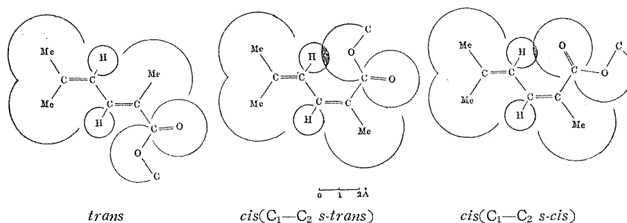
Fig. 1. Planar projection diagrams of cis - and trans - \alpha\delta -dimethylsorbic esters.
