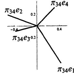
Figure 13: \{\pi_{34}e_i\}_{i=1,2,3,4} .
