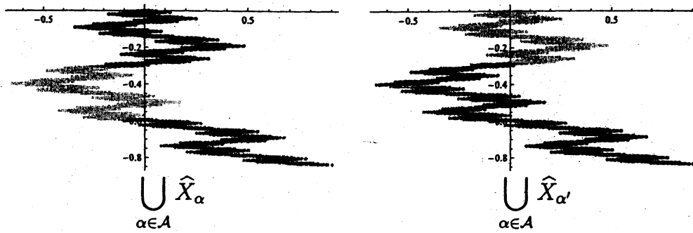
Figure 12: \bigcup_{\alpha \in \mathcal{A}} \hat{X}_\alpha and \bigcup_{\alpha \in \mathcal{A}} \hat{X}_{\alpha'} .
