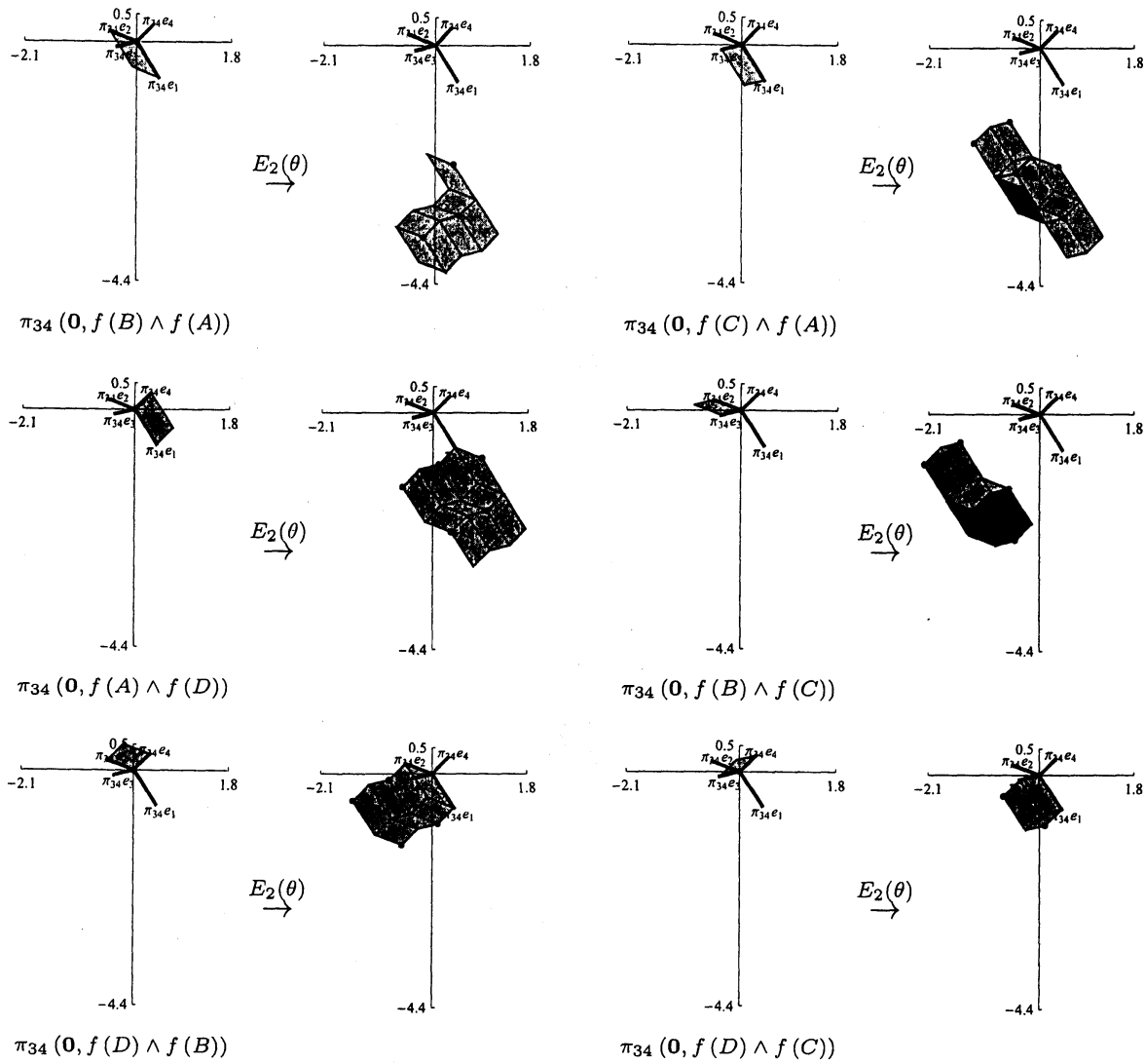
Figure 15: E_2(\theta)(0, \alpha \wedge \beta) .
