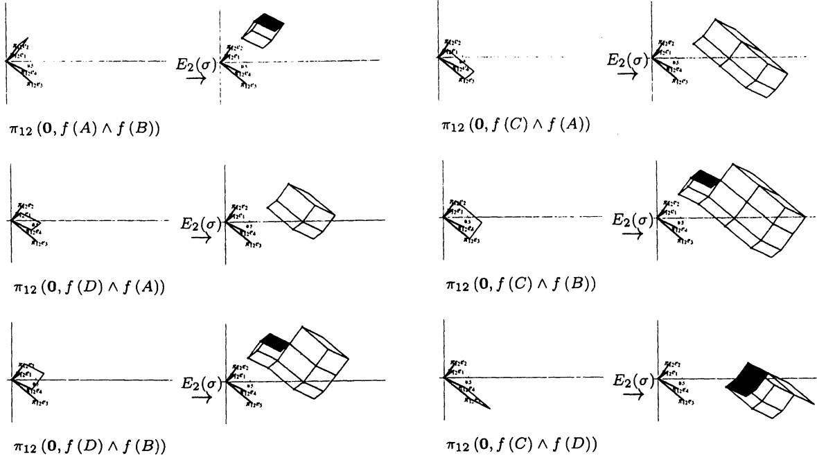
Figure 23: E_2(\sigma)(0, \alpha \wedge \beta) .
