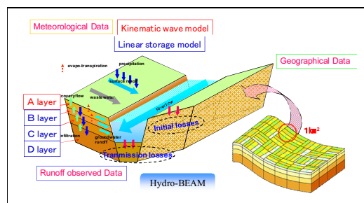
Fig. 5 Conceptual model of Hydro-BEAM
