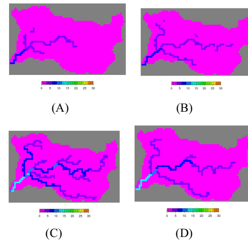
Fig. 24 Distribution maps of transmission losses in W. Assiut; (A) Early stage of surface flow, ; (B) hydrograph is rising toward the maximum peak of discharge; (C) reaching to the maximum of distribution; (D) starting the recession of surface flow to zero flow.
