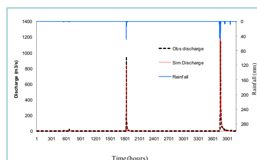
Fig. 15 Hourly hydrographs of simulated and observed discharges in wadi Al-Khoud during three infrequent events of rainfall.
