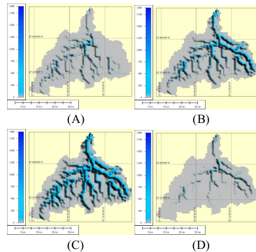
Fig. 19 Distribution maps of surface runoff of event of (Mar. 18- 2007) in W. Al-Khoud; (A) Early stage of surface flow, ; (B) hydrograph is rising toward the maximum peak of discharge; (C) reaching to the maximum of distribution; (D) starting the recession of surface flow to zero flow.
