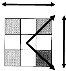
Figure 15. Binomial sequence of diagonal dynamical system
