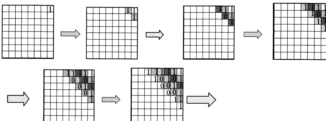
Figure 13. Binomial sequence of Sierpinski dynamical system
