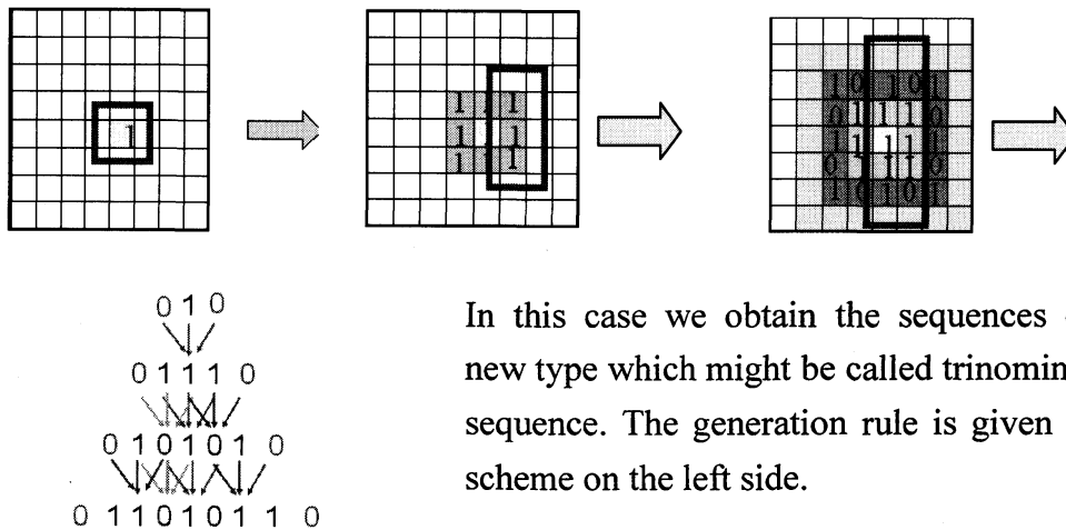
Figure 16. Trinomial sequence of Moore dynamical system
