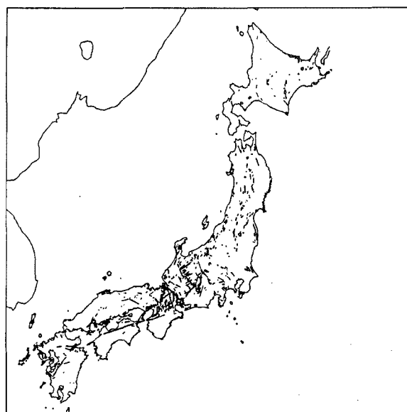
Fig. 5. Distribution of active faults in Japan.
