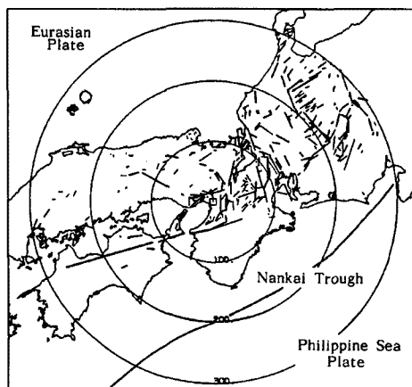
Fig. 7. Active faults in the Kinki district.
