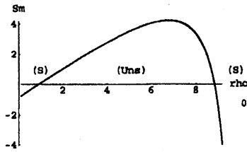
Figure 1: S_0(\rho)
