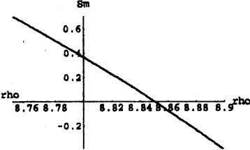
Figure 3: \rho_2^* = 8.85
