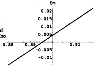
Figure 2: \rho_1^* = 0.896
