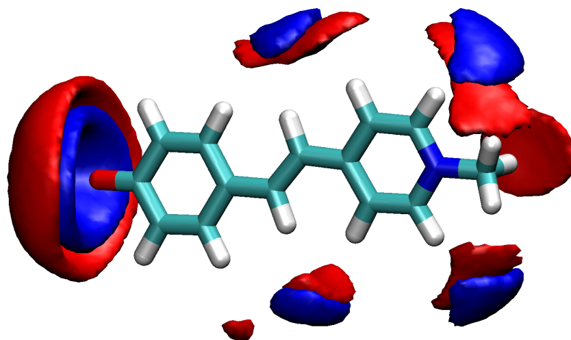
Figure 4: Spatial distribution functions of (a) water and (b) the hydroxyl group of methanol around the Brook's merocyanine obtained from the mean-field QM/MM calculations. The blue and red isosurfaces (color online) represent the regions where the number densities of the hydrogen atom and the oxygen atom of solvent molecules are five times higher than the bulk values, respectively.
