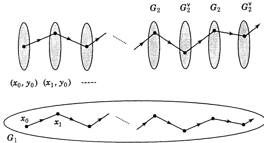
Figure 4.3: Manhattan product
