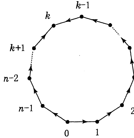
Figure 2.2: Colliding cycle
