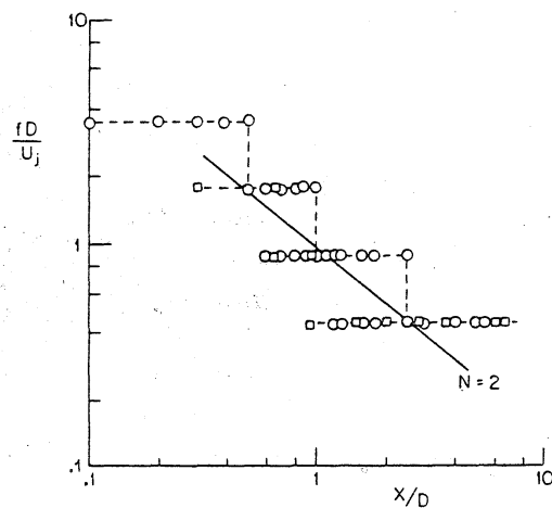
Evolution of vortex passage frequency in a forced jet (from Kihens 1980). f_c \sim f_n . R = 1 . \circ measured in shear layers; \square measured on jet centerline. — Feedback equation (Laufer & Monkewitz 1980) with N = 2 .
