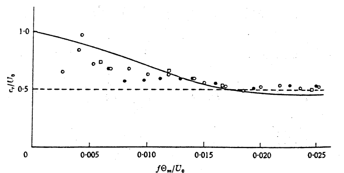
Non-dimensional phase velocity vs Strouhal number in the free boundary layer of an axisymmetric jet (○, U_0 = 8 m/sec; ●, U_0 = 4 m/sec) and of a plane jet (□, U_0 = 8 m/sec) compared with the spacewise theory (—) and the timewise theory (---) after Freymuth.
