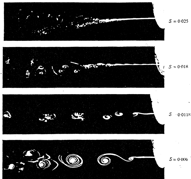
Dependence of the smoke picture on the Strouhal number. D = 7.5 \text{ cm} , U_0 = 3 \text{ m/sec} , \Delta y = 0.1 \text{ cm} .
