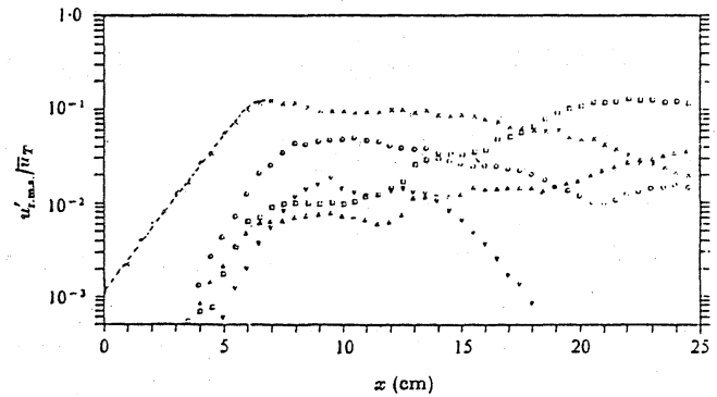
Downstream growth of u'_{r,max} maxima. Excitation at \beta = 0.222 ; R(x_0) = 145 . \times , \beta ; \circ , 2\beta ; \nabla , 3\beta ; \square , \beta/2 ; \triangle , 3\beta/2 . ---, theoretical Landau equilibration curve.
