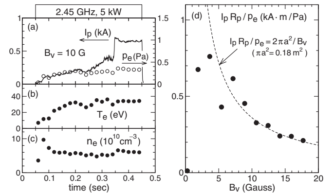
FIG. 4. (a) Temporal evolutions of plasma current ( I_p ), electron pressure ( p_e ), (b) electron temperature ( T_e ), and (c) density ( n_e ). (d) Relationship of I_p R_p / p_e versus B_v at the initial discharge stage. R_p is the plasma major radius.
