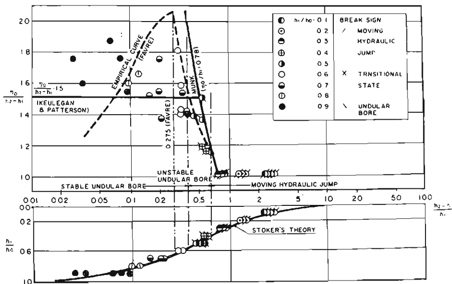
Fig. 5 Maximum height of the bore.
