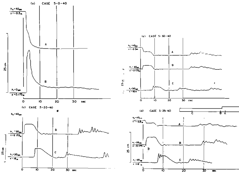
Fig. 6 The time changes of the water level.
