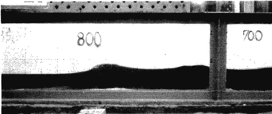
Photo. 3. Undularbore bore with spilling break ( h_1/h_0=0.5 , x=8m ).
