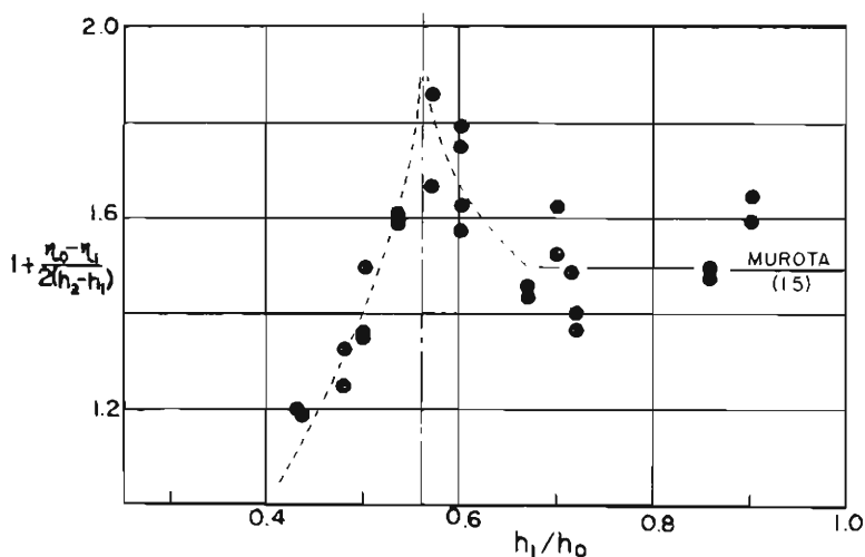
Fig. 8 Relative amplitude of the bore.
