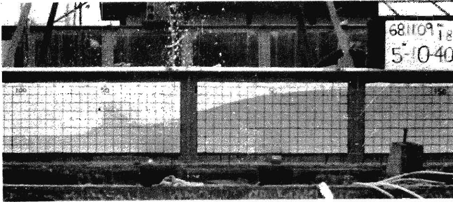
Photo. 2. Plunging break ( h_1/h_0=0.25 , x=0.5m ).
