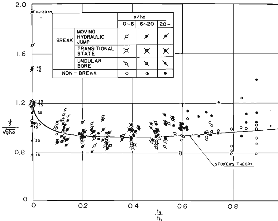
Fig. 3 The wave velocity.
