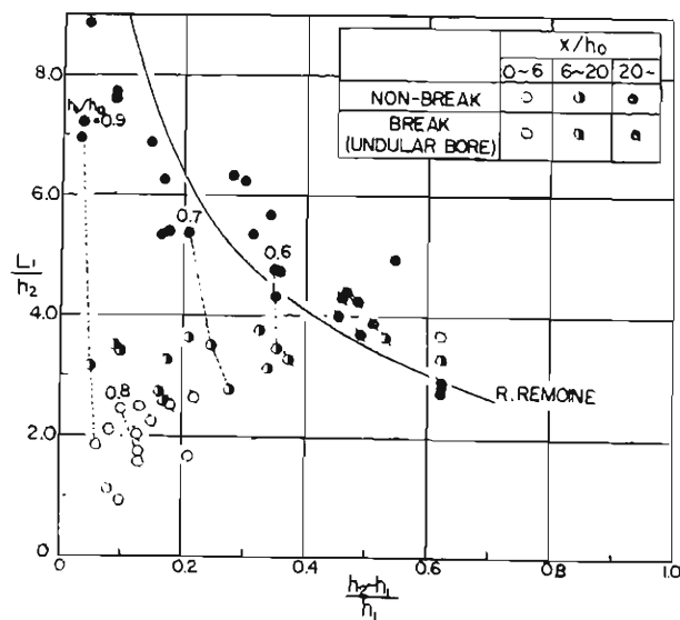
Fig. 9 The relationship between L_1 and mean wave height.
