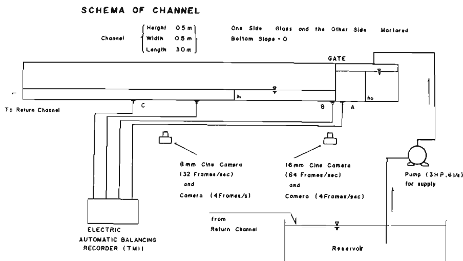
Fig. 1 Experimental apparatus.
