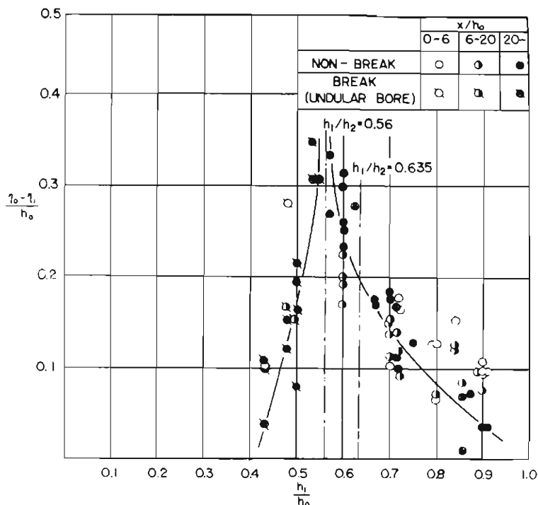
Fig. 7 The amplitude of the bore.
