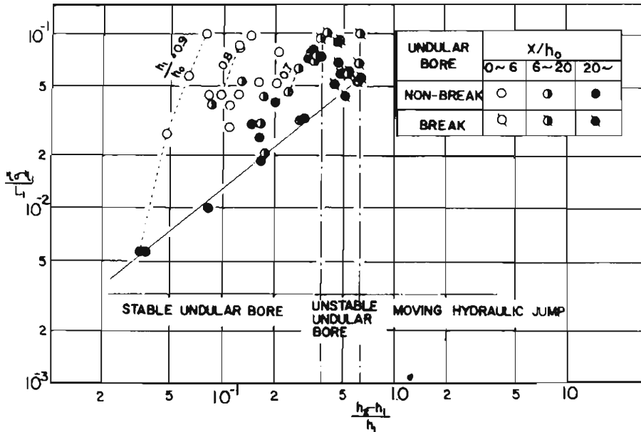
Fig. 10 The relationship between the mean wave height and (\eta_0 - \eta_1)/L_1 .
