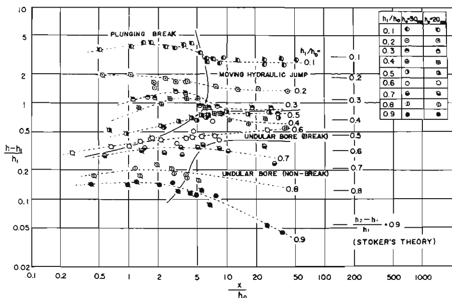
Fig. 4 Development of the bore height.
