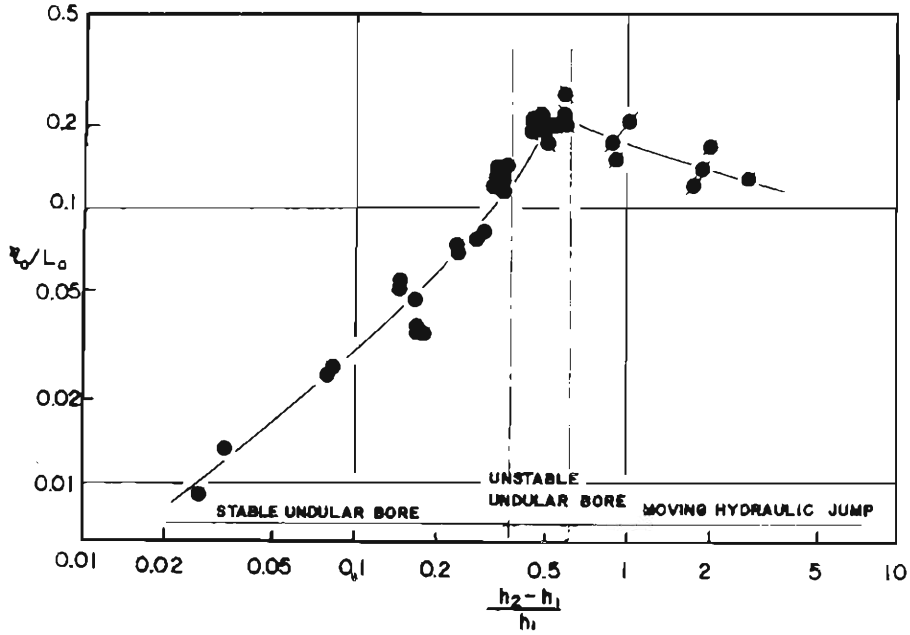
Fig. 11 The variation of \eta_0/L_0 .
