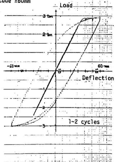
H-specimen A-12 Controlled deflection amplitude \pm 60 mm
