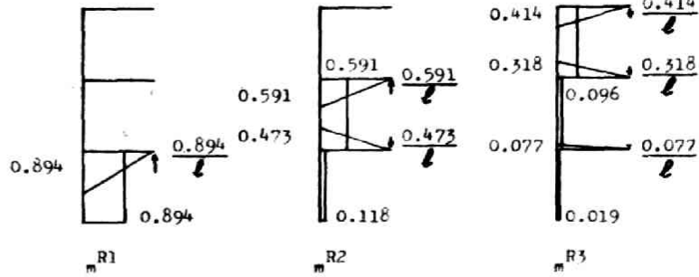
Fig.8 THE ORTHONORMAL SET OF RESIDUAL MOMENT DISTRIBUTIONS (Unit: \sqrt{2EI_1/l} )
