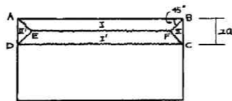
Fig. 3 Partial collapse mode C.
