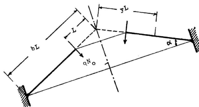
Fig.3 Clamped Truncated Conical Shell
