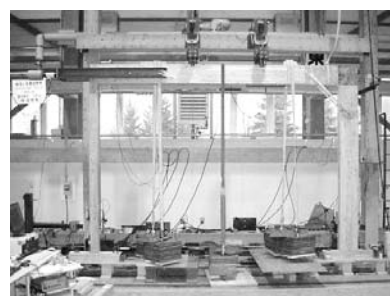
Figure 4. Portal frame racking test with dead load.
