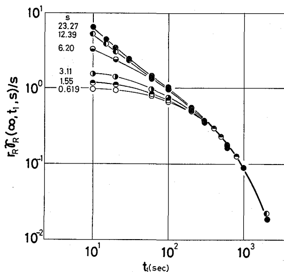
Fig. 6. Reduced plot of relative ultimate elastic recovery \gamma_R(\infty, t_1, s)/s vs. period of stress relaxation t_1 . Reduction factor r_R is determined with r_R = [\gamma_R(\infty, t_1, s)/s] / [\lim_{s \rightarrow 0} \gamma_R(\infty, t_1, s)/s] at t_1 = 1000 sec.
