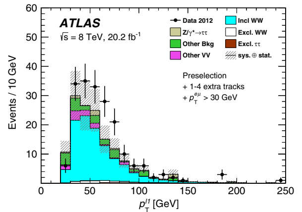
FIG. 10. The leading-lepton p_T^{\ell 1} distribution in the inclusive W^+W^- control region. The simulation includes all appropriate correction factors such as f_{1-4}^{\text{sim}} for Drell-Yan and f_{1-4}^{\text{p}} for inclusive W^+W^- production.
