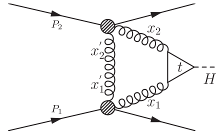
FIG. 2. The lowest-order Feynman diagram for the exclusive Higgs boson production. The variables x_1 and x_2 are the fractions of the momenta carried by the gluons that contribute to the production of the Higgs boson, with respect to the momenta of the protons P_1 and P_2 . The variables x'_1 and x'_2 , on the other hand, are the fractions of the momentum carried by the exchanged third gluon with respect to the momenta of the protons P_1 and P_2 .
