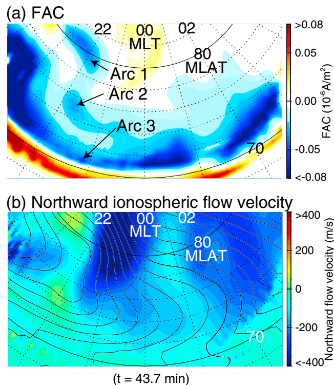
Figure 6. (a) FAC at the ionosphere (negative upward) and (b) north-south component of the ionospheric flow velocity at t = 43.7 min. The contour line indicates the ionospheric electric potential at interval of 2 kV.
