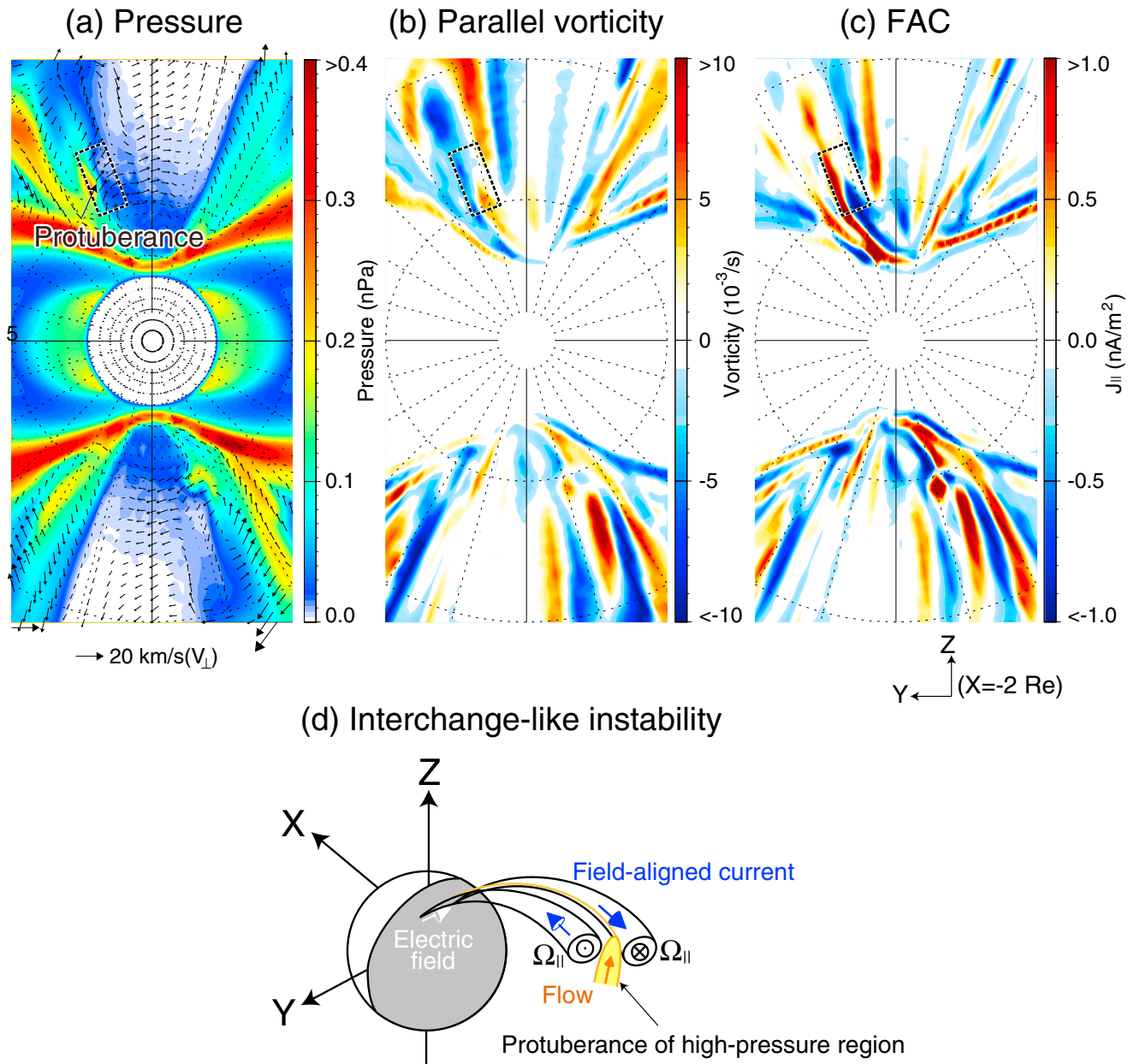
Figure 5. (a) Plasma pressure, (b) parallel vorticity \Omega_{||} , and (c) parallel current density J_{||} (negative upward in the Northern Hemisphere) in the Y-Z plane at X = -2.0 \text{ Re} at t = 3.7 \text{ min} . The arrow indicates the plasma flow velocity perpendicular to the magnetic field. (d) A schematic drawing is present to explain the possible instability taking place in the coupling between the magnetosphere and the ionosphere.
