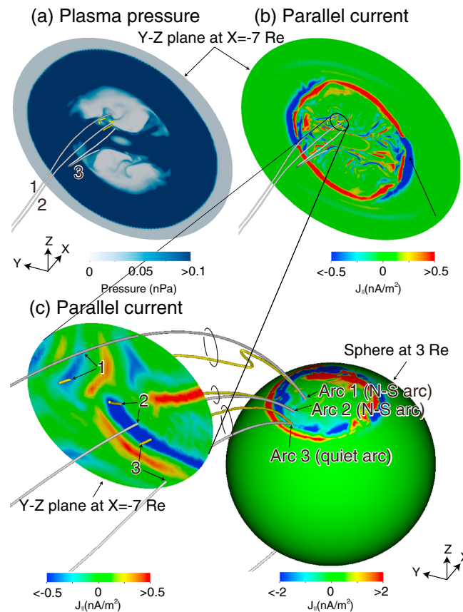
Figure 3. (a) Plasma pressure and (b and c) parallel current density in the Y-Z plane at X = -7 R_E . In (c), parallel current is also drawn on the surface at 3 R_E . The yellow and white lines indicate the current line and the magnetic field line, respectively, extending from Arcs 1, 2, and 3 at t = 43.7 min. The color codes indicate the parallel current density (negative upward in the Northern Hemisphere). We are looking down the Earth from the midnight-dawn sector in the Northern Hemisphere.
