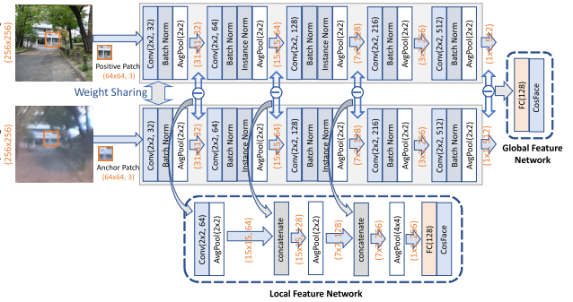
FIGURE 8. The structure of AFD-Net.
