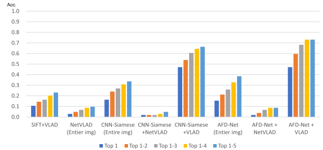
FIGURE 10. Experimental result (Accuracy comparison).
