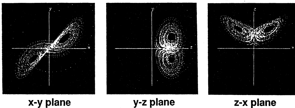
Fig.2 Lorentz attractor
