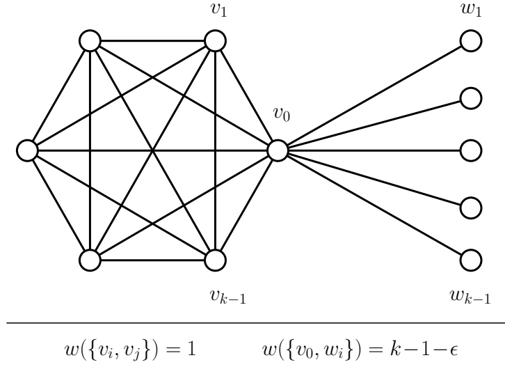
Figure 2.5: A tight example for GSA applied to k -PPG.
