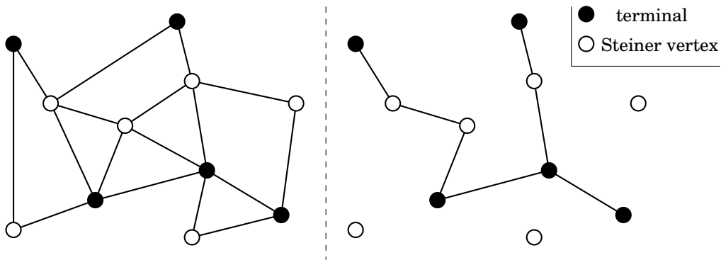
Figure 1.10: Graph and Steiner tree.
