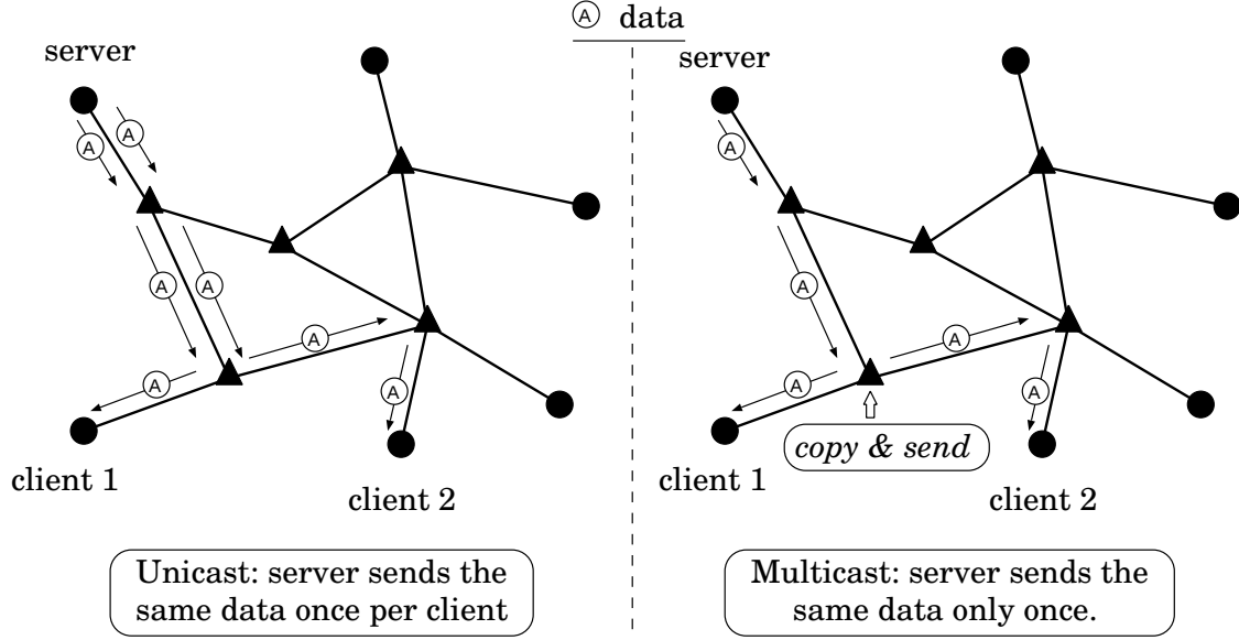
Figure 1.11: Unicast and multicast in communication network.
