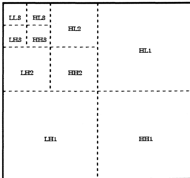
Fig.1 An example of DWT (The third stage of DWT)
