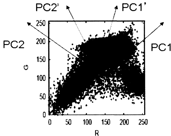
Fig.14 An example of PCA analysis (Principal Component Analysis) and slant coordinate system conversion as a preprocessing for the data hiding based on the MRA analysis.
