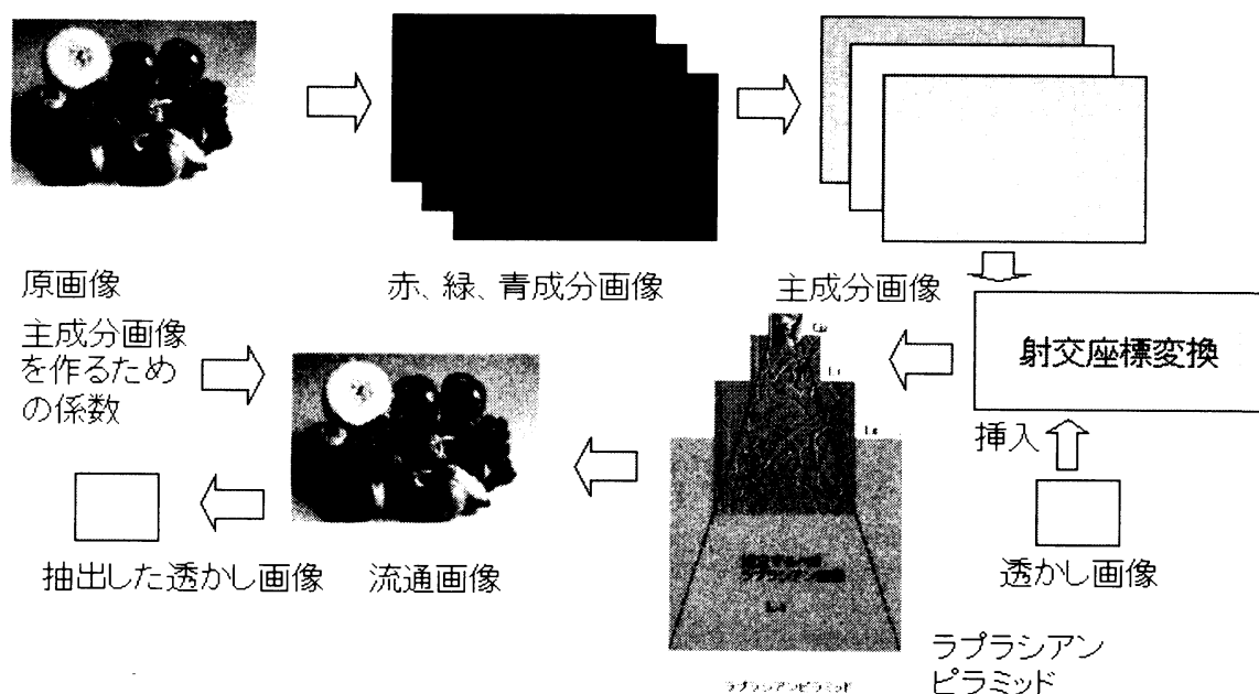
Fig.21 Process flow of the proposed data hiding with preprocessing of Principal Component Analysis and oblique coordinate system conversions
