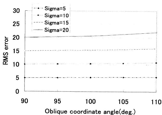
Fig.19 RMSE between oblique coordinate conversion and decompressed image and the original image when the normally distributed random noise is added.
