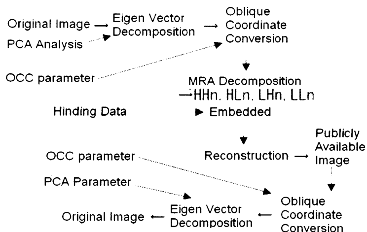
Fig.20 Process flow of data hiding based on MRA with PCA conversion and oblique coordinate system conversion.
