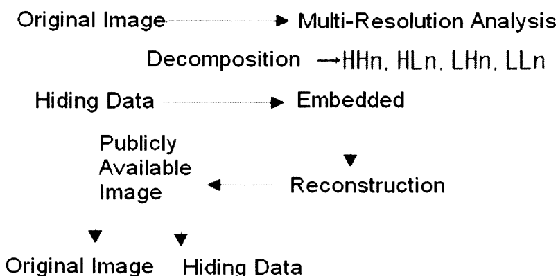
Fig.3 Process flow of data hiding based on Multi Resolution Analysis (MRA)
