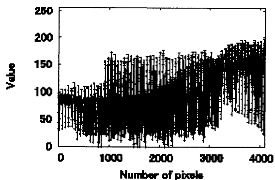
Fig.12 Hiding data
