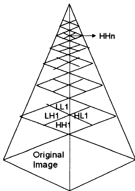
Fig.2 Laplacian pyramid
