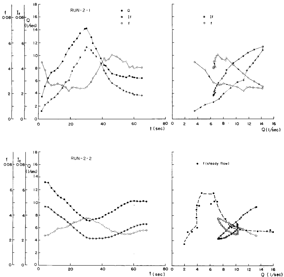
Fig. 9 Unsteady flows in the closed channel for RUN-2.
