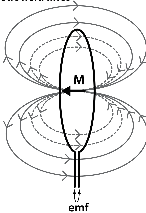
Fig. 1. A precessing magnetic moment \mathbf{M} inside a loop of conducting wire induces electromotive force (EMF) across the wire terminals. The EMF is determined by a time derivative of the net magnetic flux penetrating through the loop. Magnetic field lines that are confined in the loop, as schematically depicted by the broken lines, make no contribution to the EMF. Only field lines that take a path that returns outside the loop, as described by the solid lines, can induce EMF.
