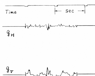
Fig 7 Here is an example of amplitude of vibro-acceleration, when the motor-truck, T_1 , went over a crossing ditch " S_{12} ". In this figure, the first peak of amplitude shows the passage of the front wheels, and the second peak (maximum amplitude) shows the passage of the rear wheels.
