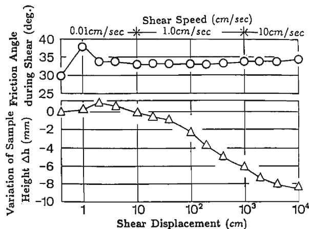
Fig. 11-1. Variation of the friction angle during shear and the sample height in the Test Series B on the Shirakawa river sand (grain size = 0.84 \sim 9.52 \text{ mm} ). Normal stress \sigma = 3.0 \text{ kgf/cm}^2 . Void ratio during shear e = 0.56 \sim 0.76 .
