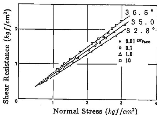
Fig. 3. Result of the ring shear tests on the unsaturated Jizukiyama landslide soil. Degree of saturation =20.8\sim26.1\% . Void ratio during shear e=0.71\sim0.86 . (Fukuoka et al. 24 ).
