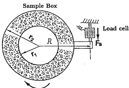
Fig. 6. Shear plane of the sample and the load cell for measurement of the shear resistance.
