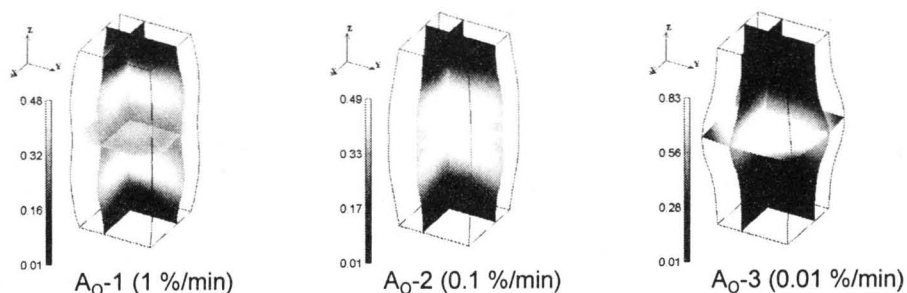
Figure 7.25 Distribution of \gamma^p inside of the specimen for the A_O cases with different strain rates (Axial strain: 20%)
