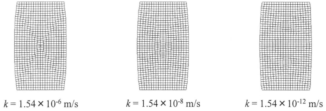
Figure 3.7 Deformed mesh at an average axial strain of 7%
