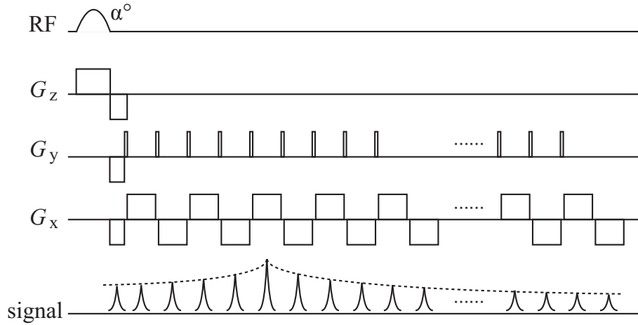
Figure 2.7: The pulse sequence of the echo planar imaging.
