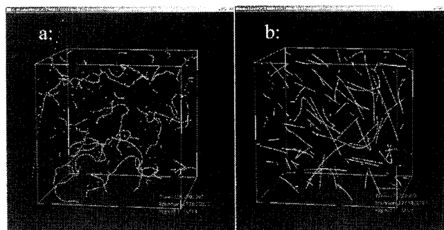
Fig.1 Snapshot of calculation for pair charged particles a: Calculation by Ewald method. b: Calculation by reaction filed method.
