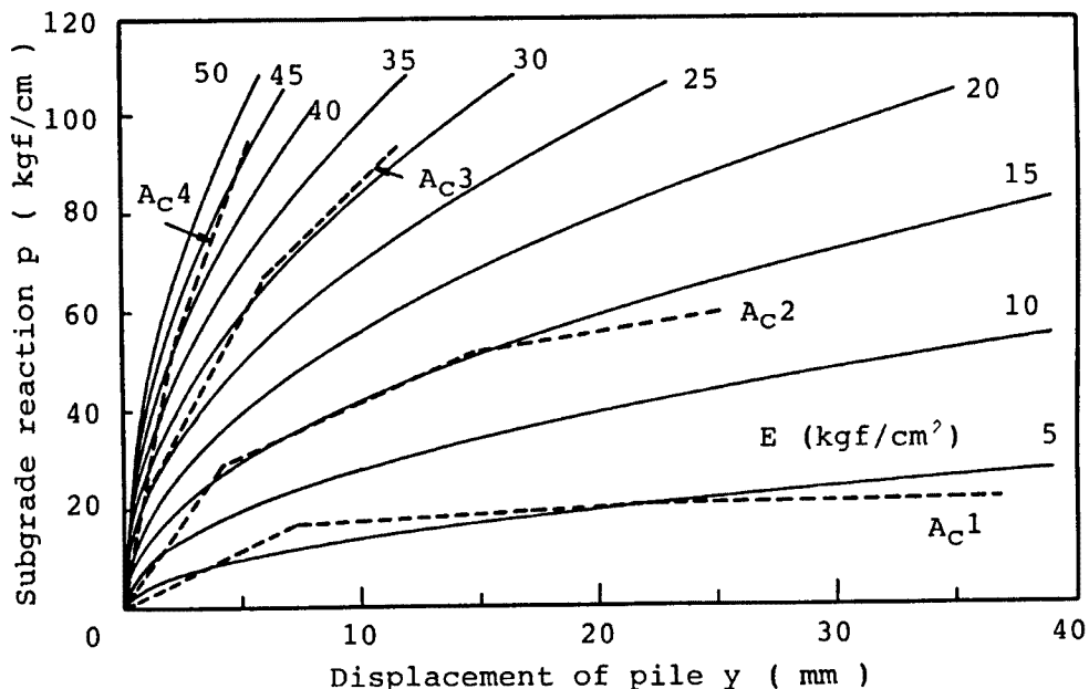
Fig. 12. Relationship between subgrade reaction ( p ) and displacement of pile ( y ), p \sim y curves.
