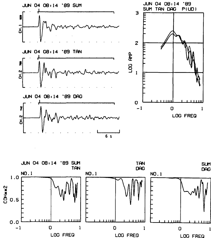
Fig. 6. Coherences for P waves from the deep event shown in Fig. 5.
