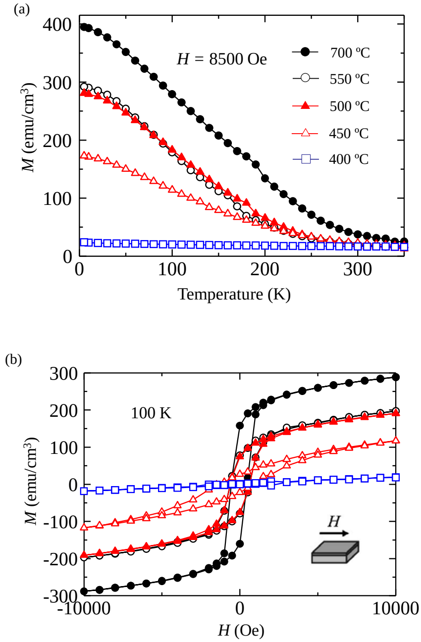
Fig. 2.7 (a) M - T curves for the thin films with ordered and disordered phases. The external magnetic field of 8500 Oe was applied parallel to the film surface. (b) M - H curves at 100 K.
