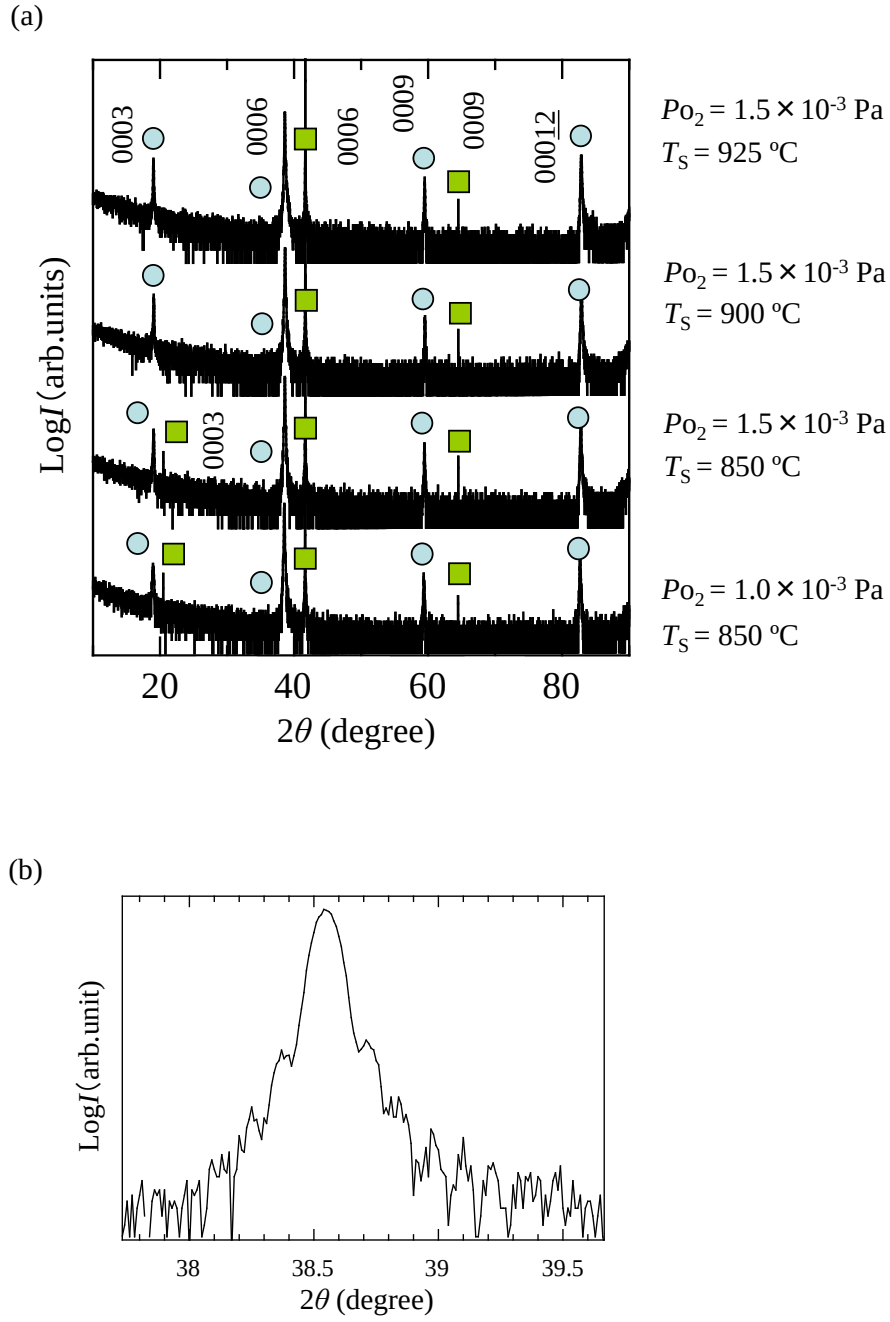
Fig. 3.1 (a) Out-of-plane XRD patterns for \text{FeTiO}_3\text{--Fe}_2\text{O}_3 solid solution thin films grown at various deposition conditions; \circ : ordered-phase of solid solution, \blacksquare : \alpha\text{-Al}_2\text{O}_3 . (b) Magnified image of 0006 peak for thin film grown at P_{O_2} = 1.5 \times 10^{-3} Pa and T_S = 925 °C.
