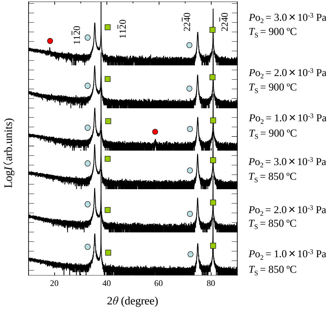
Fig. 4.3 Out-of-plane (A-plane) XRD patterns of FeTiO 3 -Fe 2 O 3 thin films grown on \alpha -Al 2 O 3 (1120) substrates; ■ : \alpha -Al 2 O 3 substrate, ● : FeTiO 3 -Fe 2 O 3 , ● : impurities.
