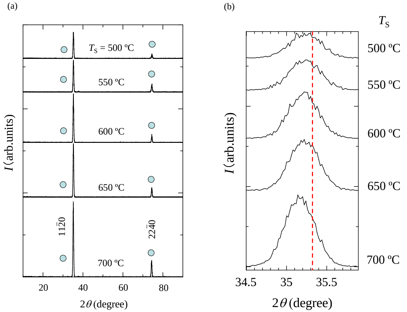
Fig. 2.5 (a) In-plane XRD patterns for solid solution thin films grown at T_s = 500\text{--}700\text{ }^{\circ}\text{C} ; \bullet : ordered phase. (b) Magnified image of 11\bar{2}0 peaks displayed in Fig. 2.5 (a).
