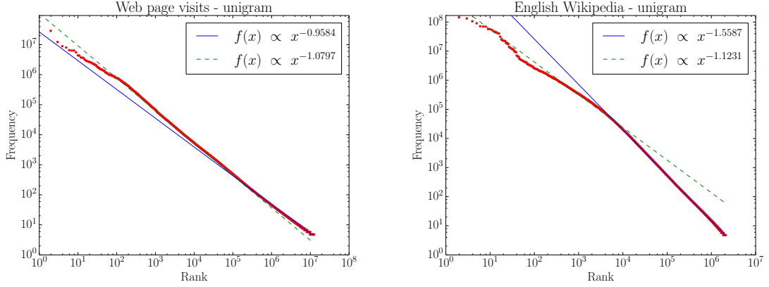
Figure 5.2: Log-log plot for Web page visit data (left) and English Wikipedia data (right). X-axis represents rank of activity or words in frequency table, and y-axis is number of occurrences. Solid and dashed lines represent regression lines for all data and early part of the data (rank less than 10^4 ), respectively.
