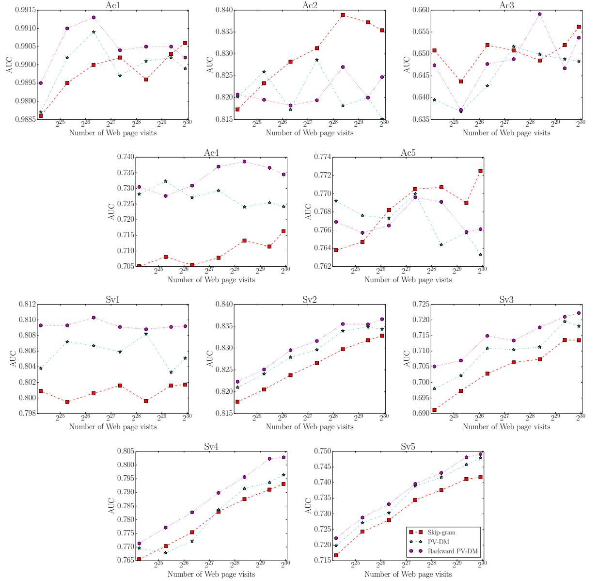
Figure 5.8: Experimental results when changing the number of Web site visits in learning the vector models. Horizontal axis (number of Web site visits) is logarithmic scale.
