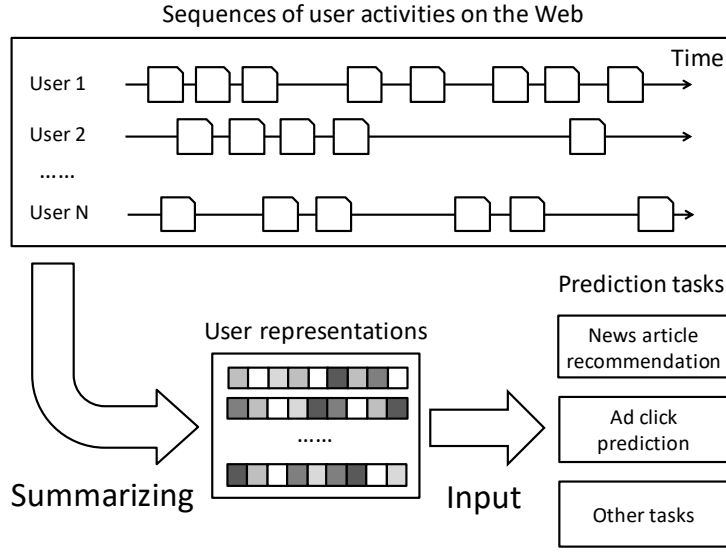
Figure 5.1: Overview of our approach. Low-dimensional vectors, in which sequences of user activities are summarized, are used as common features among various user-related prediction tasks. Note that targets of prediction tasks, such as ad clicks, do not need to be included in sequences.
