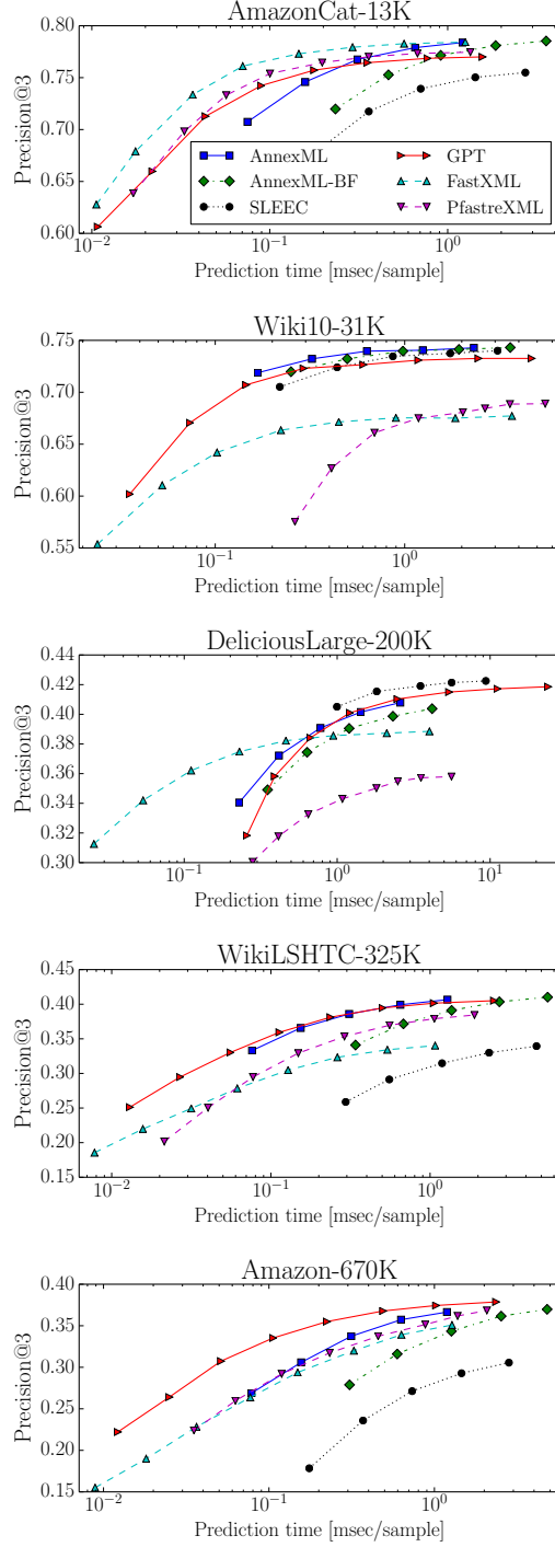
Figure 1: Precision@3 versus prediction time when the number of learners changes.
