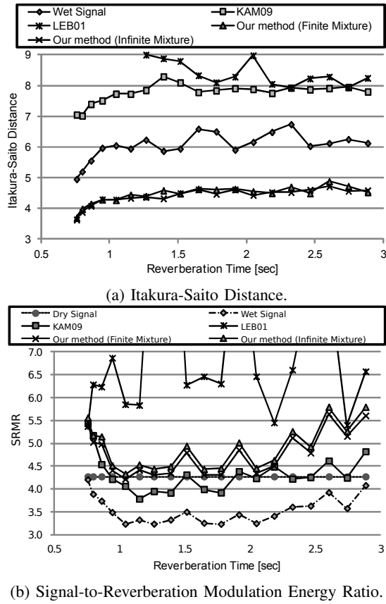
Fig. 5: Evaluation measures of synthetic impulse response as the reverberation time is varied.
