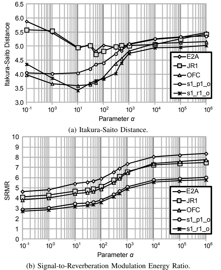
Fig. 6: Evaluation measures as \alpha is varied.
